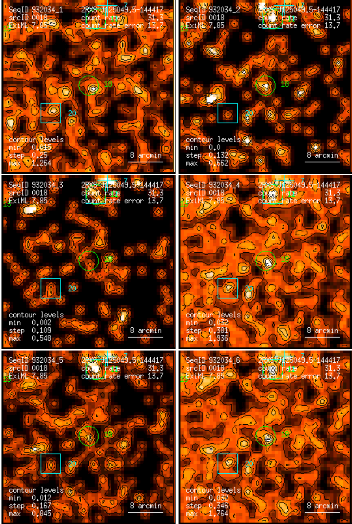
Figure 18: RASS 932034: detection 0018: band rate images, Gaussian filter: (1) PSPC channels 11 – 41, (2) 52 – 90, (3) 91 – 201, (4) 11 – 235, (5) 52 – 201, (6) 11 – 201. Broad band rates in counts/ks. Band rate contour levels in counts/ks/arcmin 2 .
