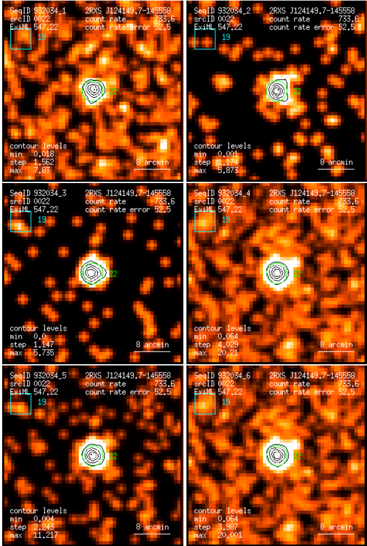
Figure 22: RASS 932034: detection 0022: band rate images, Gaussian filter: (1) PSPC channels 11 – 41, (2) 52 – 90, (3) 91 – 201, (4) 11 – 235, (5) 52 – 201, (6) 11 – 201. Broad band rates in counts/ks. Band rate contour levels in counts/ks/arcmin 2 .
