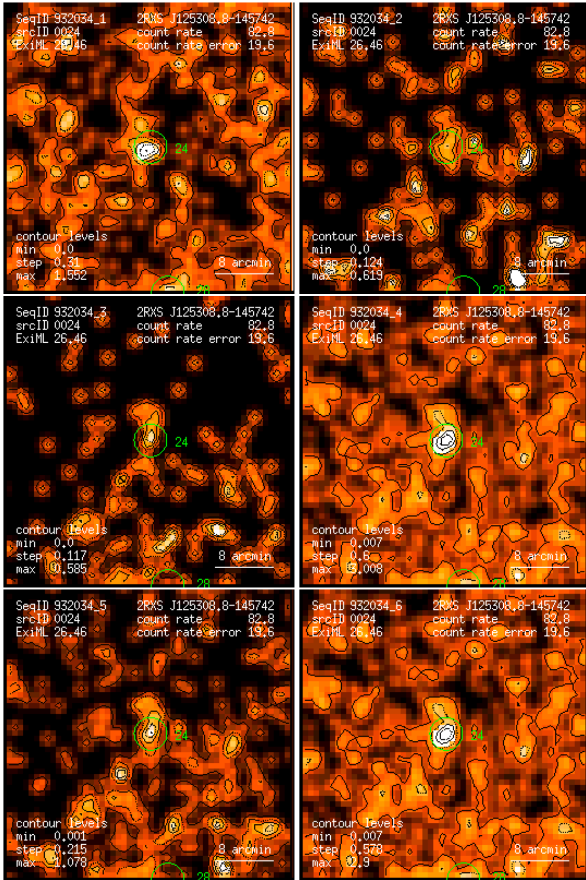
Figure 24: RASS 932034: detection 0024: band rate images, Gaussian filter: (1) PSPC channels 11 – 41, (2) 52 – 90, (3) 91 – 201, (4) 11 – 235, (5) 52 – 201, (6) 11 – 201. Broad band rates in counts/ks. Band rate contour levels in counts/ks/arcmin 2 .
