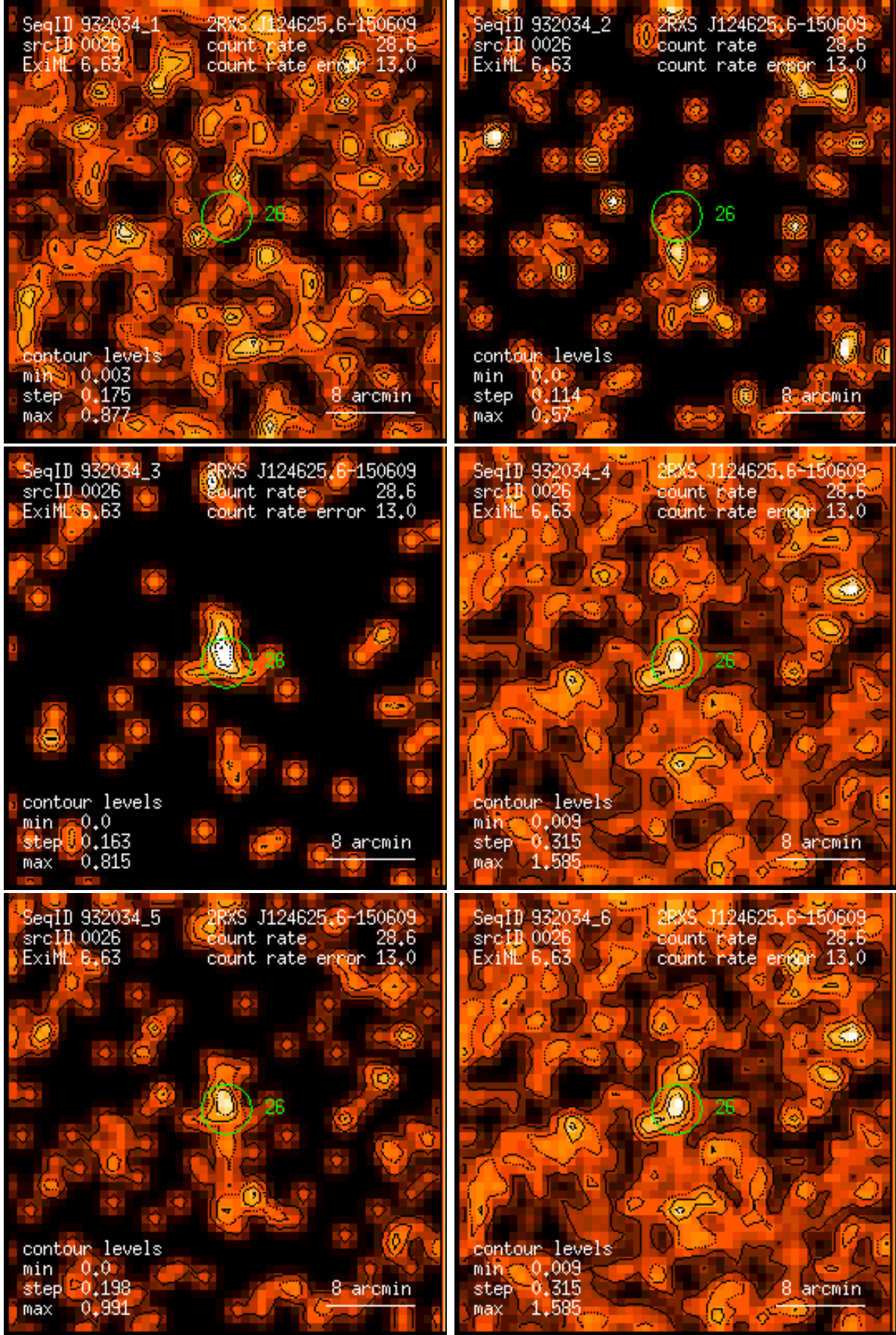
Figure 26: RASS 932034: detection 0026: band rate images, Gaussian filter: (1) PSPC channels 11 – 41, (2) 52 – 90, (3) 91 – 201, (4) 11 – 235, (5) 52 – 201, (6) 11 – 201. Broad band rates in counts/ks. Band rate contour levels in counts/ks/arcmin 2 .
