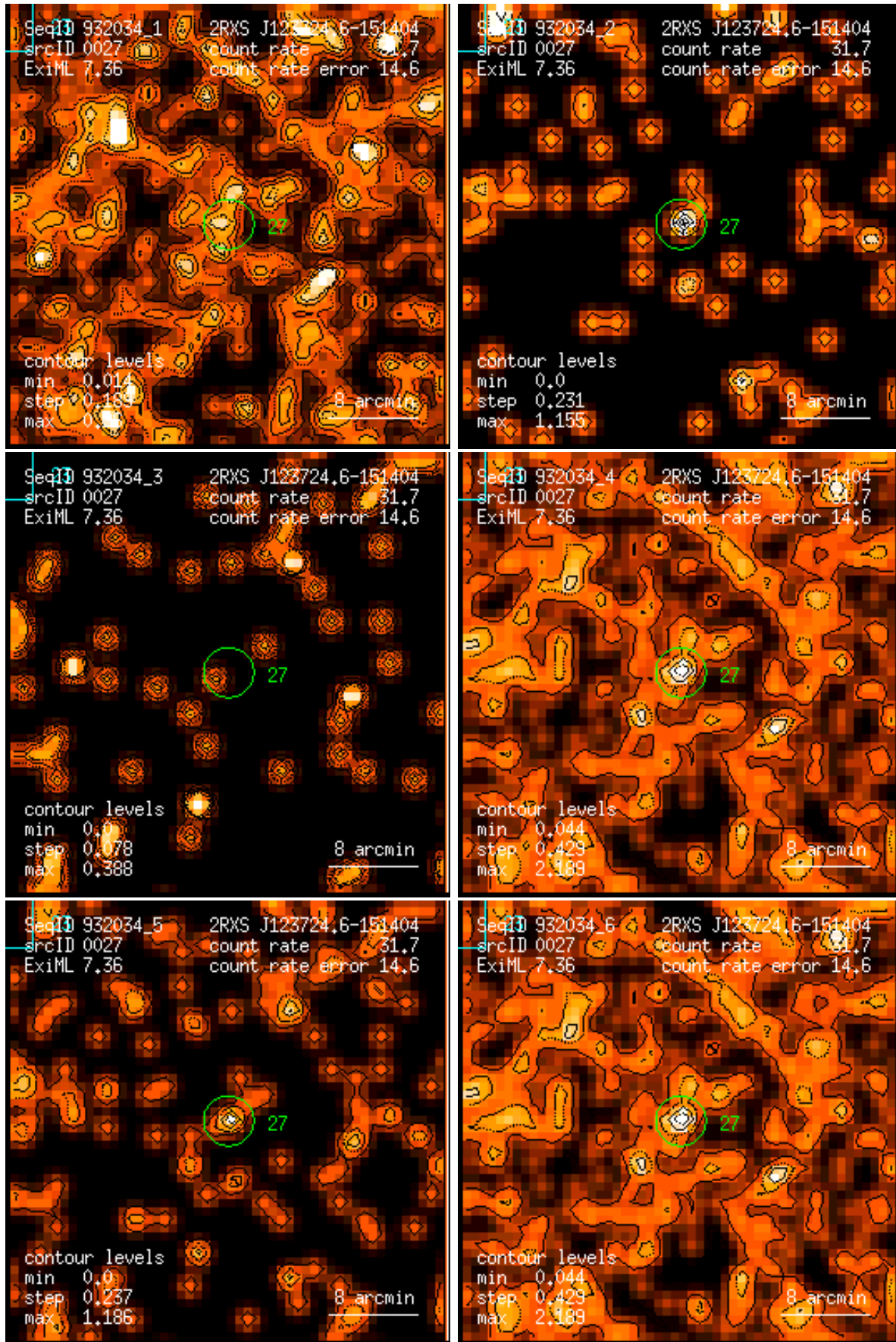
Figure 27: RASS 932034: detection 0027: band rate images, Gaussian filter: (1) PSPC channels 11 – 41, (2) 52 – 90, (3) 91 – 201, (4) 11 – 235, (5) 52 – 201, (6) 11 – 201. Broad band rates in counts/ks. Band rate contour levels in counts/ks/arcmin 2 .
