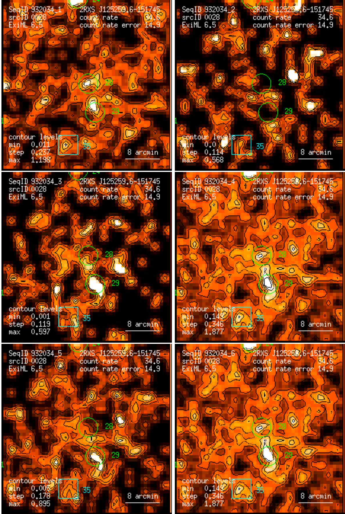
Figure 28: RASS 932034: detection 0028: band rate images, Gaussian filter: (1) PSPC channels 11 – 41, (2) 52 – 90, (3) 91 – 201, (4) 11 – 235, (5) 52 – 201, (6) 11 – 201. Broad band rates in counts/ks. Band rate contour levels in counts/ks/arcmin 2 .
