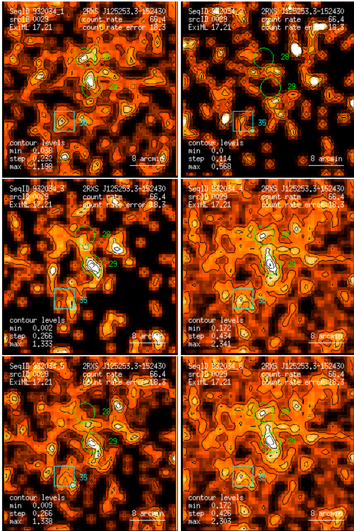
Figure 29: RASS 932034: detection 0029: band rate images, Gaussian filter: (1) PSPC channels 11 – 41, (2) 52 – 90, (3) 91 – 201, (4) 11 – 235, (5) 52 – 201, (6) 11 – 201. Broad band rates in counts/ks. Band rate contour levels in counts/ks/arcmin 2 .
