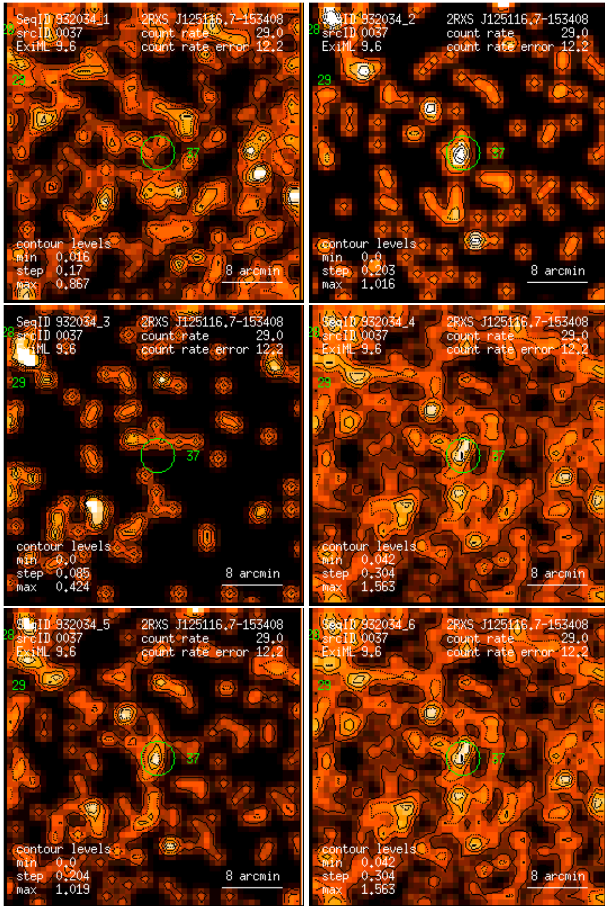
Figure 37: RASS 932034: detection 0037: band rate images, Gaussian filter: (1) PSPC channels 11 – 41, (2) 52 – 90, (3) 91 – 201, (4) 11 – 235, (5) 52 – 201, (6) 11 – 201. Broad band rates in counts/ks. Band rate contour levels in counts/ks/arcmin 2 .
