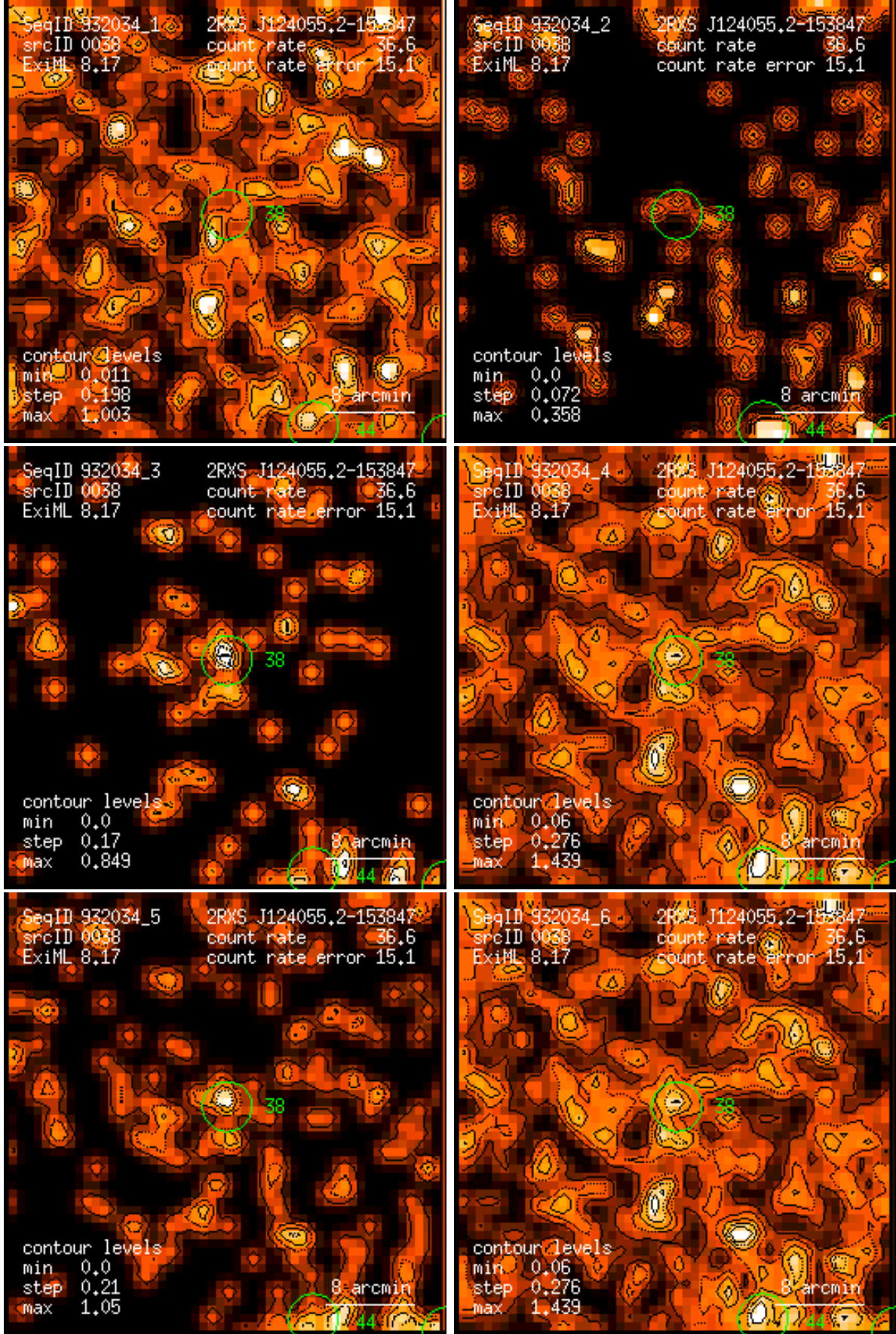
Figure 38: RASS 932034: detection 0038: band rate images, Gaussian filter: (1) PSPC channels 11 – 41, (2) 52 – 90, (3) 91 – 201, (4) 11 – 235, (5) 52 – 201, (6) 11 – 201. Broad band rates in counts/ks. Band rate contour levels in counts/ks/arcmin 2 .
