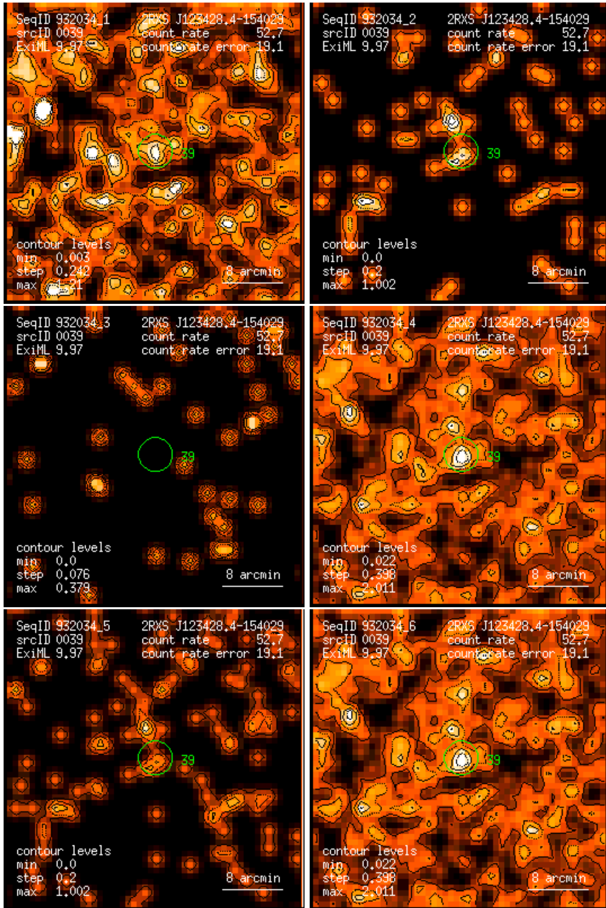
Figure 39: RASS 932034: detection 0039: band rate images, Gaussian filter: (1) PSPC channels 11 – 41, (2) 52 – 90, (3) 91 – 201, (4) 11 – 235, (5) 52 – 201, (6) 11 – 201. Broad band rates in counts/ks. Band rate contour levels in counts/ks/arcmin 2 .
