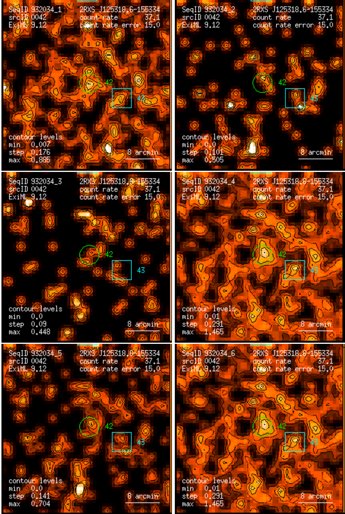
Figure 42: RASS 932034: detection 0042: band rate images, Gaussian filter: (1) PSPC channels 11 – 41, (2) 52 – 90, (3) 91 – 201, (4) 11 – 235, (5) 52 – 201, (6) 11 – 201. Broad band rates in counts/ks. Band rate contour levels in counts/ks/arcmin 2 .
