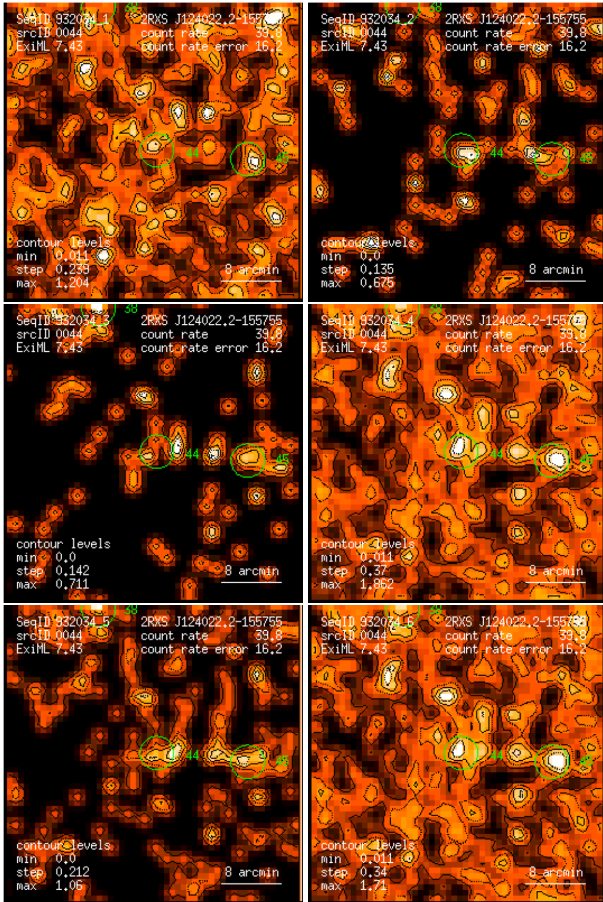
Figure 44: RASS 932034: detection 0044: band rate images, Gaussian filter: (1) PSPC channels 11 – 41, (2) 52 – 90, (3) 91 – 201, (4) 11 – 235, (5) 52 – 201, (6) 11 – 201. Broad band rates in counts/ks. Band rate contour levels in counts/ks/arcmin 2 .
