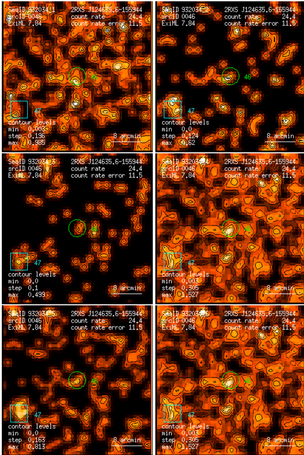
Figure 46: RASS 932034: detection 0046: band rate images, Gaussian filter: (1) PSPC channels 11 – 41, (2) 52 – 90, (3) 91 – 201, (4) 11 – 235, (5) 52 – 201, (6) 11 – 201. Broad band rates in counts/ks. Band rate contour levels in counts/ks/arcmin 2 .
