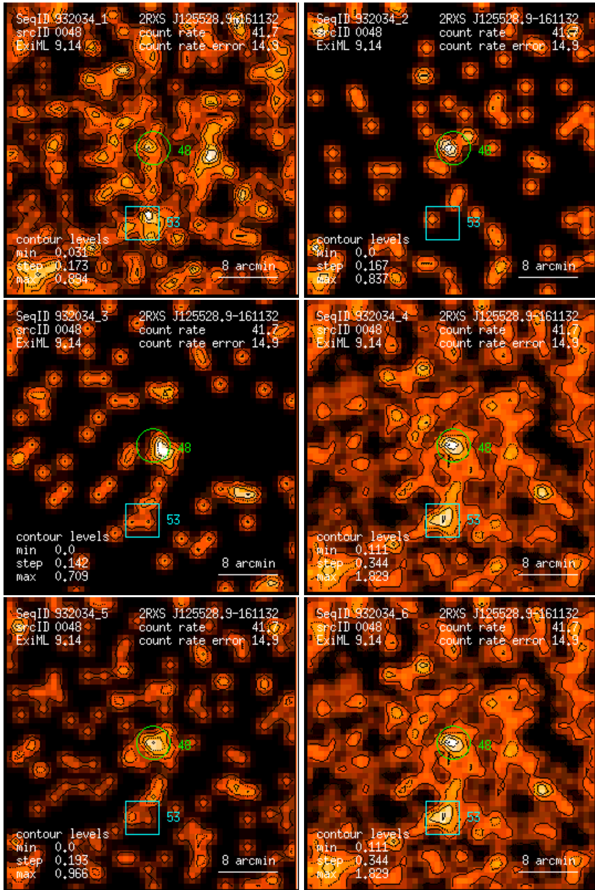
Figure 48: RASS 932034: detection 0048: band rate images, Gaussian filter: (1) PSPC channels 11 – 41, (2) 52 – 90, (3) 91 – 201, (4) 11 – 235, (5) 52 – 201, (6) 11 – 201. Broad band rates in counts/ks. Band rate contour levels in counts/ks/arcmin 2 .
