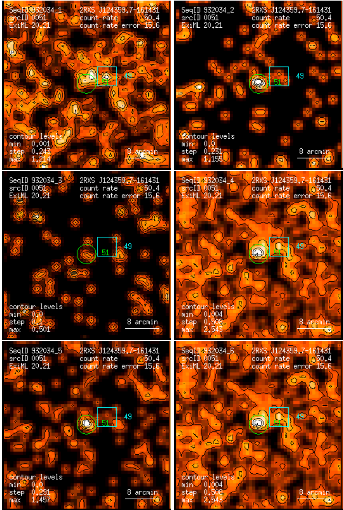
Figure 51: RASS 932034: detection 0051: band rate images, Gaussian filter: (1) PSPC channels 11 – 41, (2) 52 – 90, (3) 91 – 201, (4) 11 – 235, (5) 52 – 201, (6) 11 – 201. Broad band rates in counts/ks. Band rate contour levels in counts/ks/arcmin 2 .
