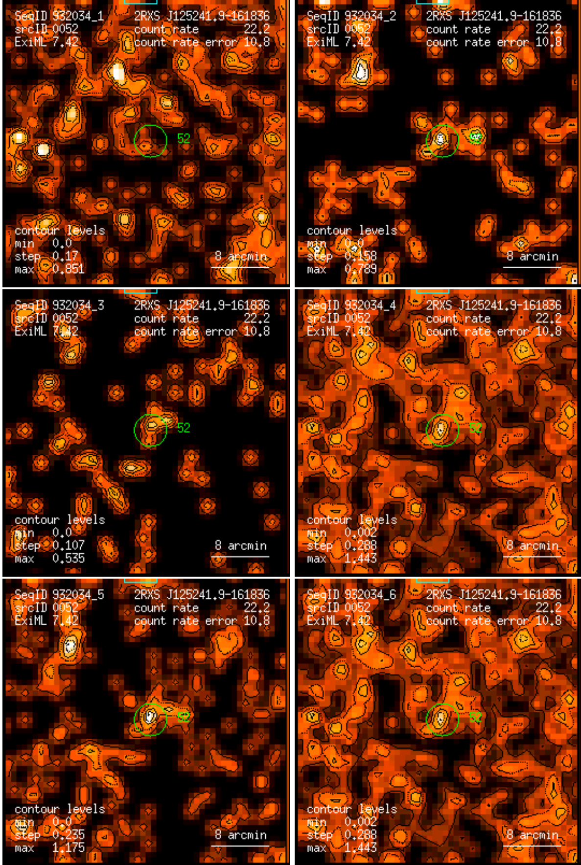
Figure 52: RASS 932034: detection 0052: band rate images, Gaussian filter: (1) PSPC channels 11 – 41, (2) 52 – 90, (3) 91 – 201, (4) 11 – 235, (5) 52 – 201, (6) 11 – 201. Broad band rates in counts/ks. Band rate contour levels in counts/ks/arcmin 2 .
