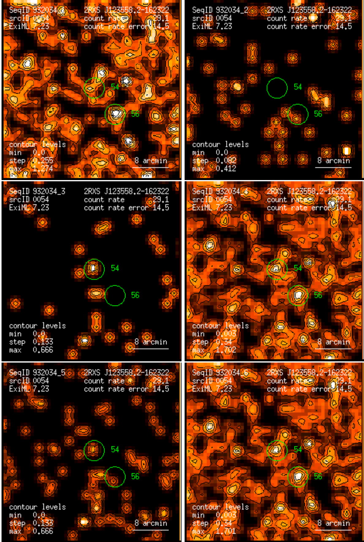
Figure 54: RASS 932034: detection 0054: band rate images, Gaussian filter: (1) PSPC channels 11 – 41, (2) 52 – 90, (3) 91 – 201, (4) 11 – 235, (5) 52 – 201, (6) 11 – 201. Broad band rates in counts/ks. Band rate contour levels in counts/ks/arcmin 2 .
