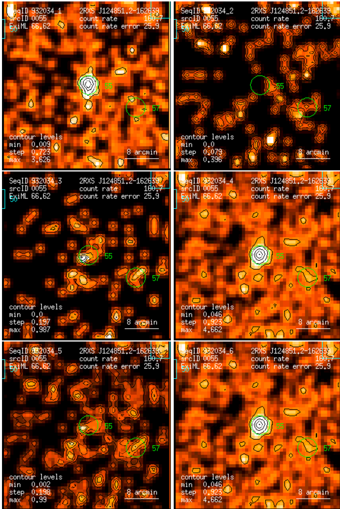
Figure 55: RASS 932034: detection 0055: band rate images, Gaussian filter: (1) PSPC channels 11 – 41, (2) 52 – 90, (3) 91 – 201, (4) 11 – 235, (5) 52 – 201, (6) 11 – 201. Broad band rates in counts/ks. Band rate contour levels in counts/ks/arcmin 2 .
