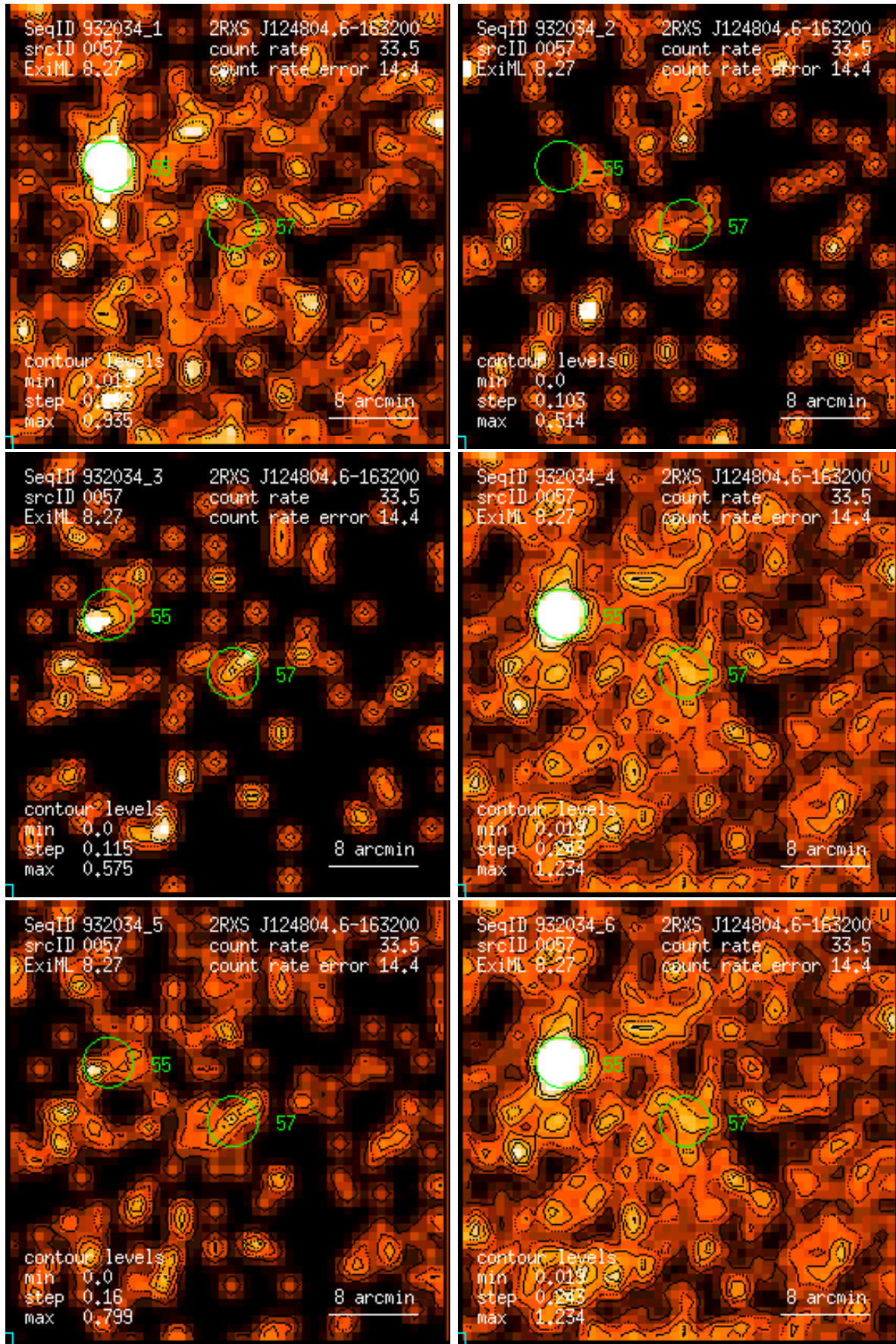
Figure 57: RASS 932034: detection 0057: band rate images, Gaussian filter: (1) PSPC channels 11 – 41, (2) 52 – 90, (3) 91 – 201, (4) 11 – 235, (5) 52 – 201, (6) 11 – 201. Broad band rates in counts/ks. Band rate contour levels in counts/ks/arcmin 2 .
