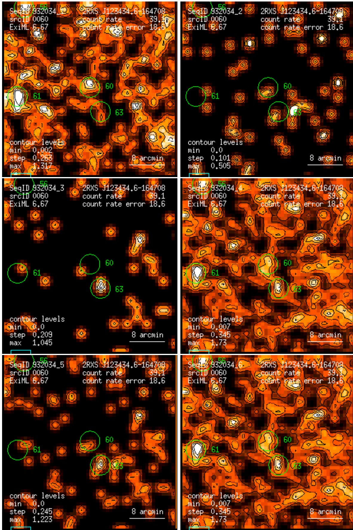
Figure 60: RASS 932034: detection 0060: band rate images, Gaussian filter: (1) PSPC channels 11 – 41, (2) 52 – 90, (3) 91 – 201, (4) 11 – 235, (5) 52 – 201, (6) 11 – 201. Broad band rates in counts/ks. Band rate contour levels in counts/ks/arcmin 2 .
