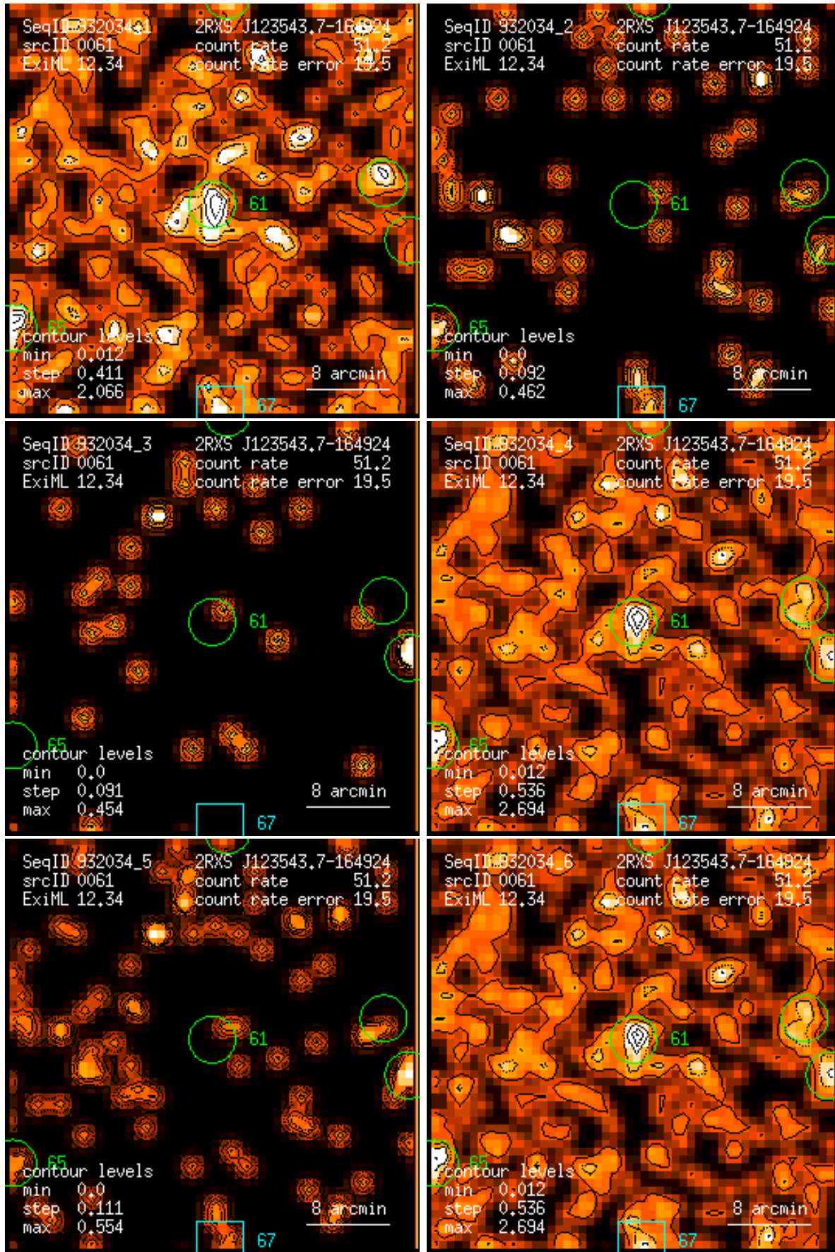
Figure 61: RASS 932034: detection 0061: band rate images, Gaussian filter: (1) PSPC channels 11 – 41, (2) 52 – 90, (3) 91 – 201, (4) 11 – 235, (5) 52 – 201, (6) 11 – 201. Broad band rates in counts/ks. Band rate contour levels in counts/ks/arcmin 2 .
