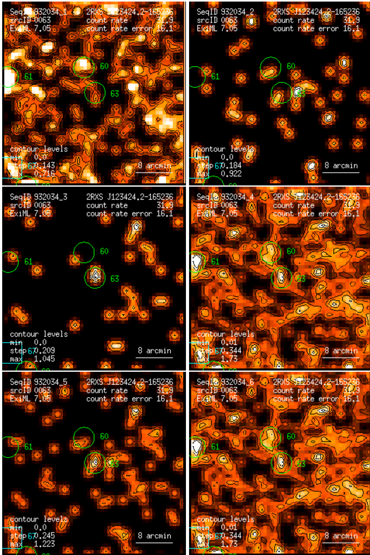
Figure 63: RASS 932034: detection 0063: band rate images, Gaussian filter: (1) PSPC channels 11 – 41, (2) 52 – 90, (3) 91 – 201, (4) 11 – 235, (5) 52 – 201, (6) 11 – 201. Broad band rates in counts/ks. Band rate contour levels in counts/ks/arcmin 2 .
