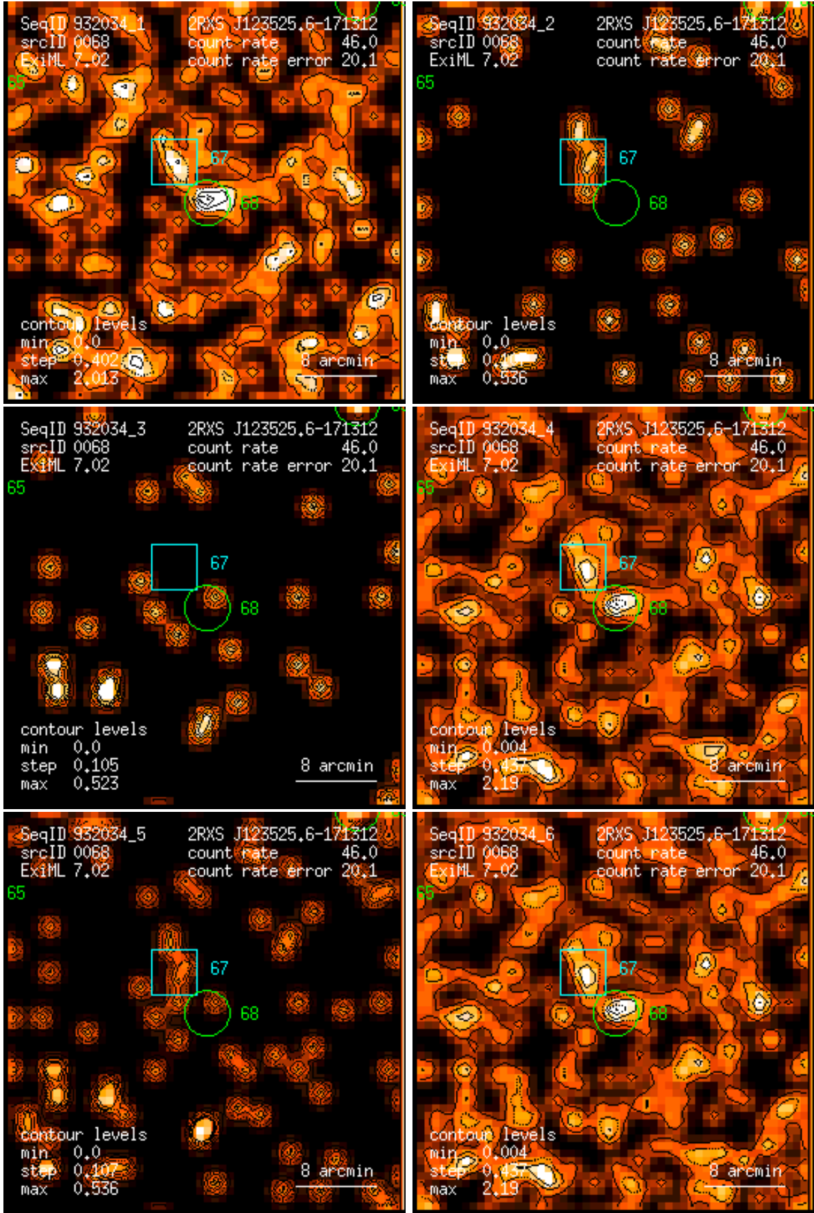
Figure 68: RASS 932034: detection 0068: band rate images, Gaussian filter: (1) PSPC channels 11 – 41, (2) 52 – 90, (3) 91 – 201, (4) 11 – 235, (5) 52 – 201, (6) 11 – 201. Broad band rates in counts/ks. Band rate contour levels in counts/ks/arcmin 2 .
