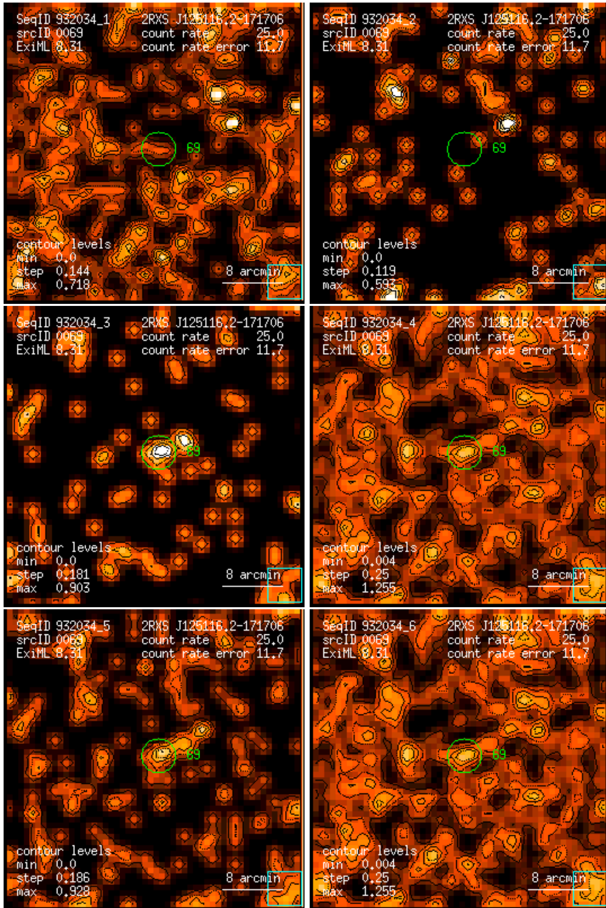
Figure 69: RASS 932034: detection 0069: band rate images, Gaussian filter: (1) PSPC channels 11 – 41, (2) 52 – 90, (3) 91 – 201, (4) 11 – 235, (5) 52 – 201, (6) 11 – 201. Broad band rates in counts/ks. Band rate contour levels in counts/ks/arcmin 2 .
