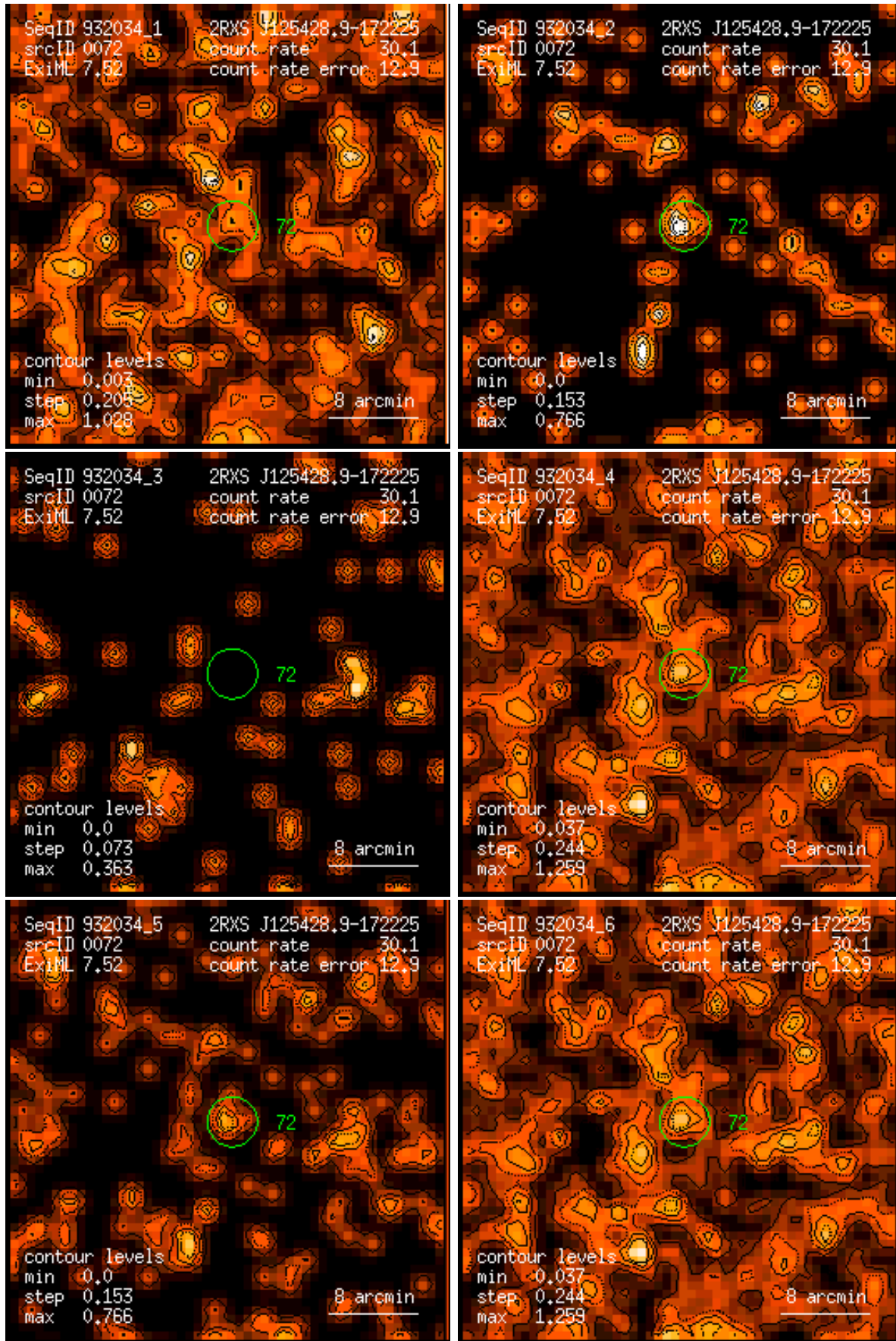
Figure 72: RASS 932034: detection 0072: band rate images, Gaussian filter: (1) PSPC channels 11 – 41, (2) 52 – 90, (3) 91 – 201, (4) 11 – 235, (5) 52 – 201, (6) 11 – 201. Broad band rates in counts/ks. Band rate contour levels in counts/ks/arcmin 2 .
