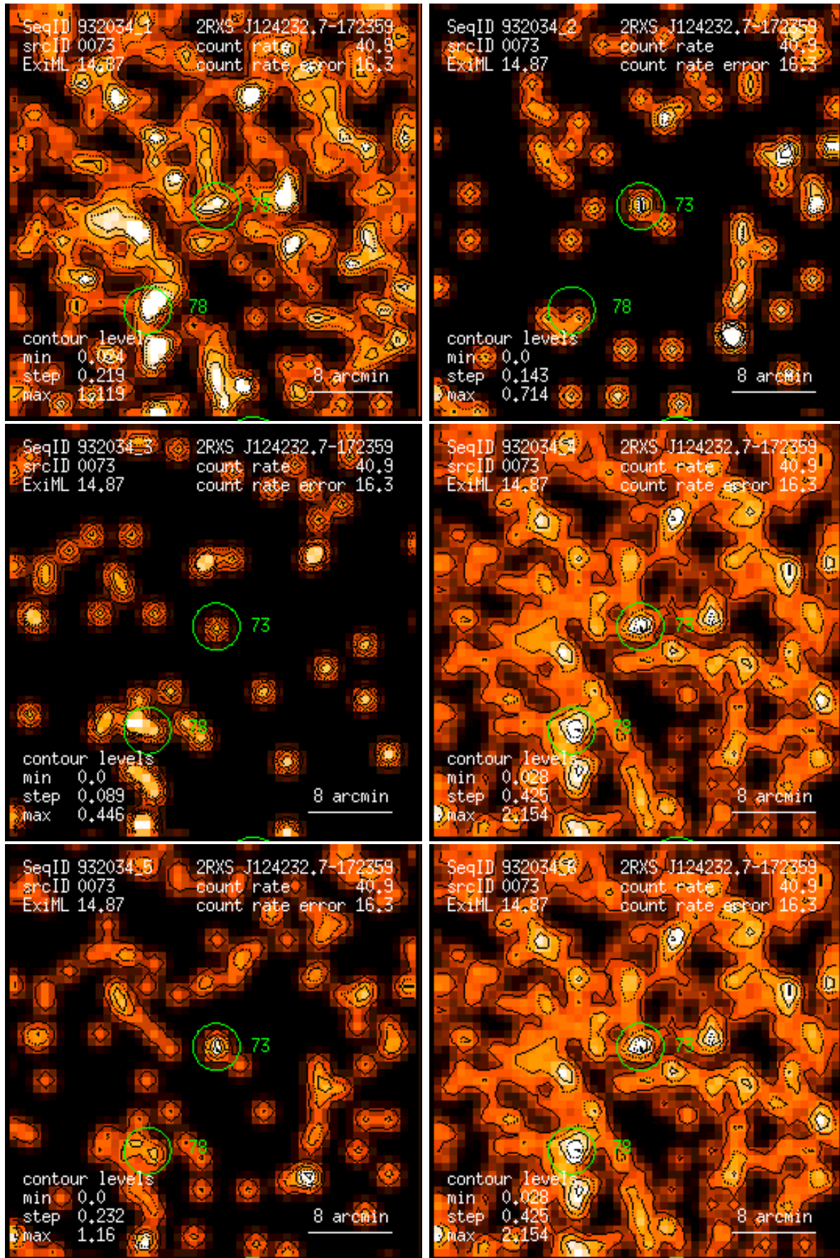
Figure 73: RASS 932034: detection 0073: band rate images, Gaussian filter: (1) PSPC channels 11 – 41, (2) 52 – 90, (3) 91 – 201, (4) 11 – 235, (5) 52 – 201, (6) 11 – 201. Broad band rates in counts/ks. Band rate contour levels in counts/ks/arcmin 2 .
