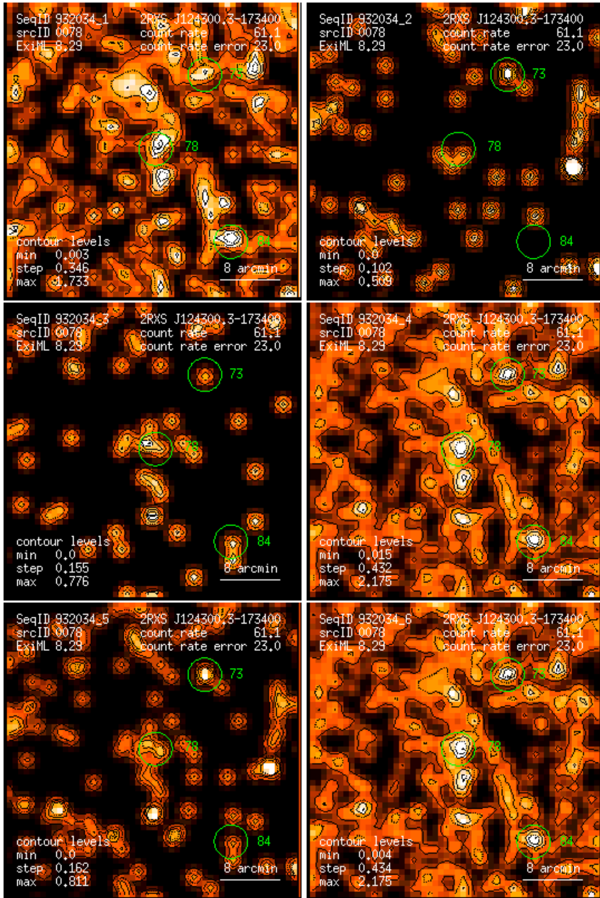
Figure 78: RASS 932034: detection 0078: band rate images, Gaussian filter: (1) PSPC channels 11 – 41, (2) 52 – 90, (3) 91 – 201, (4) 11 – 235, (5) 52 – 201, (6) 11 – 201. Broad band rates in counts/ks. Band rate contour levels in counts/ks/arcmin 2 .
