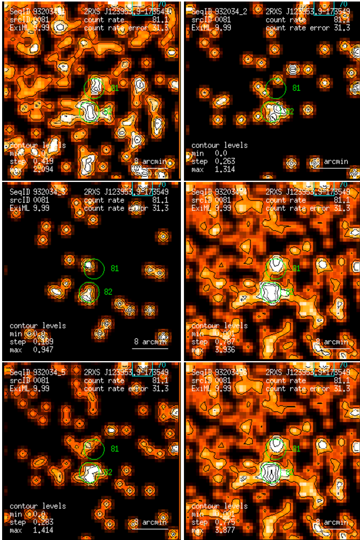
Figure 81: RASS 932034: detection 0081: band rate images, Gaussian filter: (1) PSPC channels 11 – 41, (2) 52 – 90, (3) 91 – 201, (4) 11 – 235, (5) 52 – 201, (6) 11 – 201. Broad band rates in counts/ks. Band rate contour levels in counts/ks/arcmin 2 .
