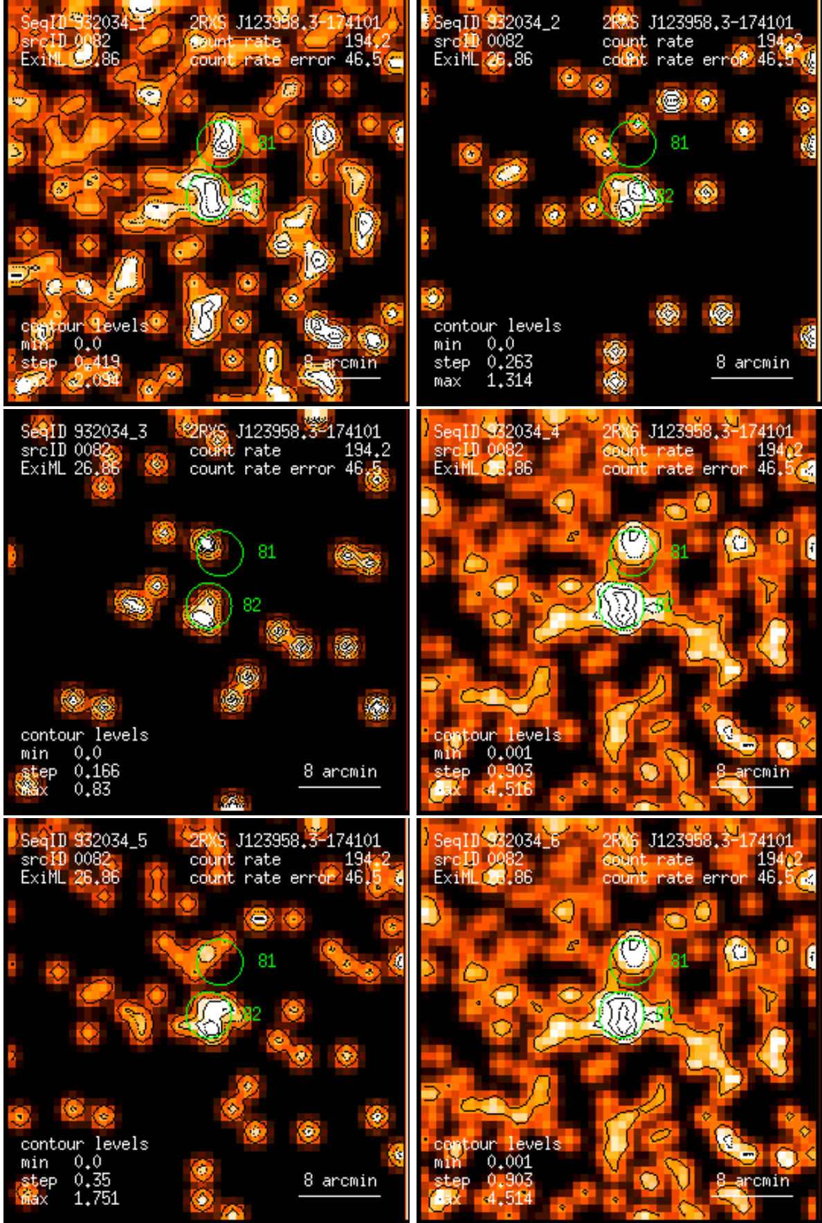
Figure 82: RASS 932034: detection 0082: band rate images, Gaussian filter: (1) PSPC channels 11 – 41, (2) 52 – 90, (3) 91 – 201, (4) 11 – 235, (5) 52 – 201, (6) 11 – 201. Broad band rates in counts/ks. Band rate contour levels in counts/ks/arcmin 2 .
