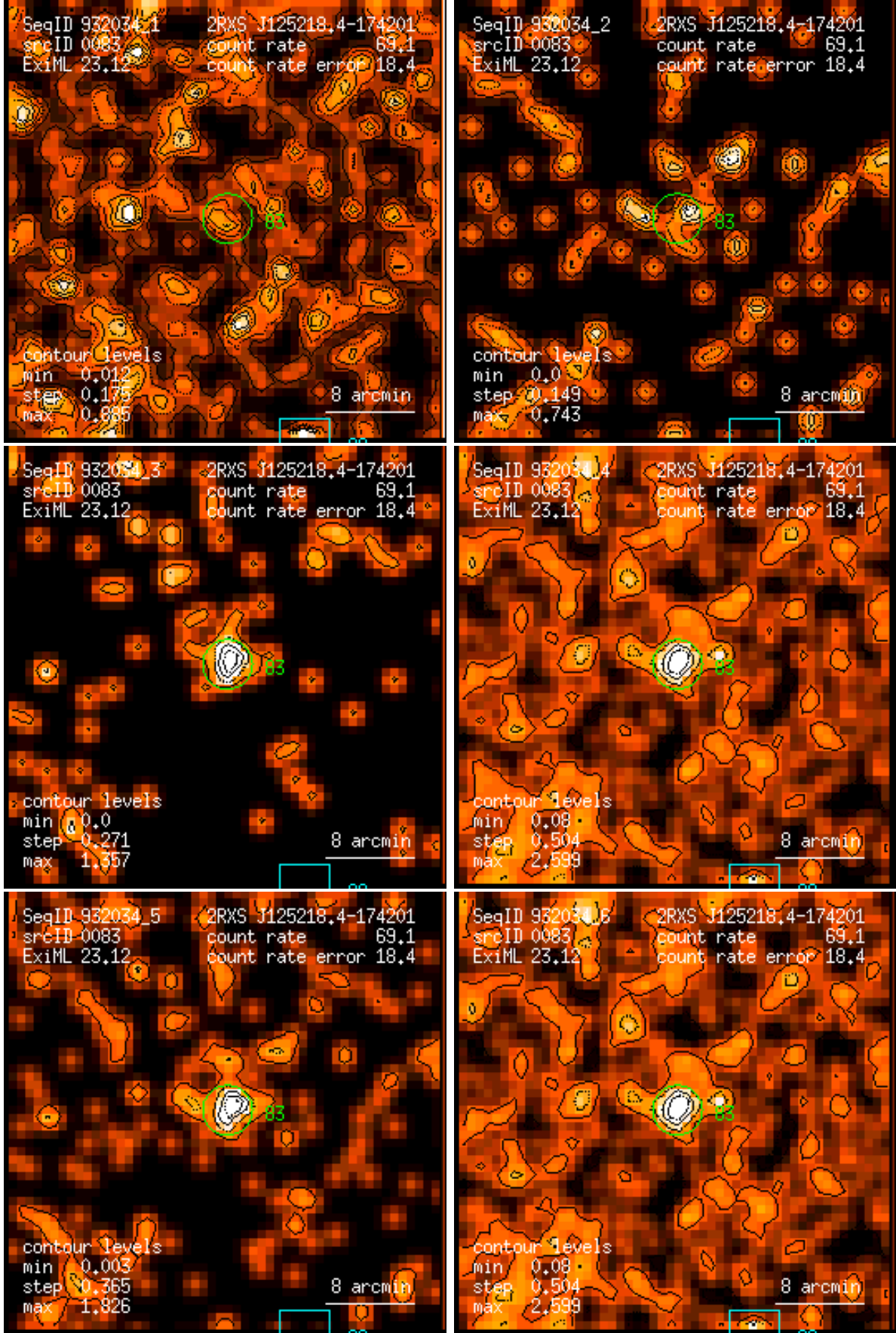
Figure 83: RASS 932034: detection 0083: band rate images, Gaussian filter: (1) PSPC channels 11 – 41, (2) 52 – 90, (3) 91 – 201, (4) 11 – 235, (5) 52 – 201, (6) 11 – 201. Broad band rates in counts/ks. Band rate contour levels in counts/ks/arcmin 2 .
