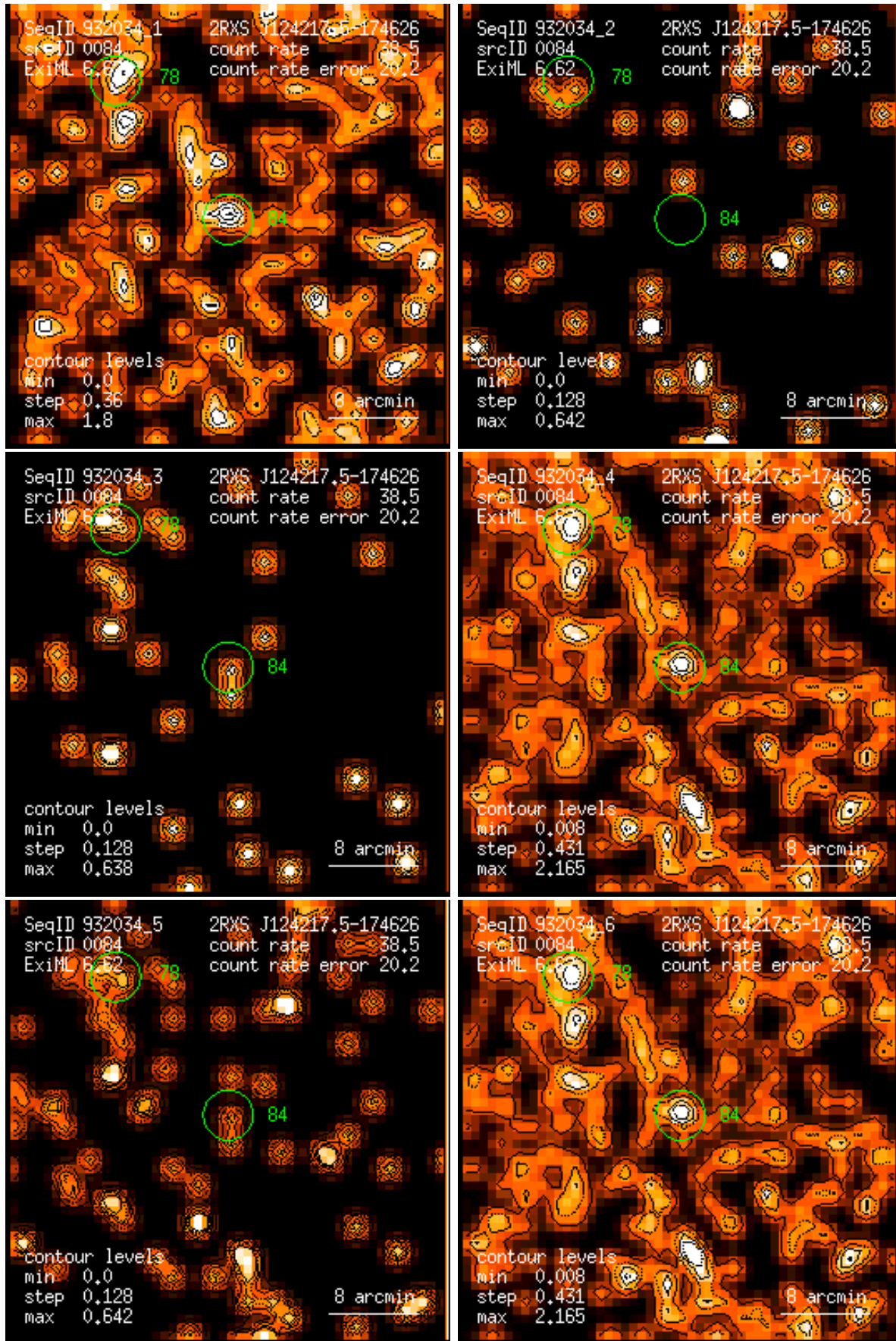
Figure 84: RASS 932034: detection 0084: band rate images, Gaussian filter: (1) PSPC channels 11 – 41, (2) 52 – 90, (3) 91 – 201, (4) 11 – 235, (5) 52 – 201, (6) 11 – 201. Broad band rates in counts/ks. Band rate contour levels in counts/ks/arcmin 2 .
