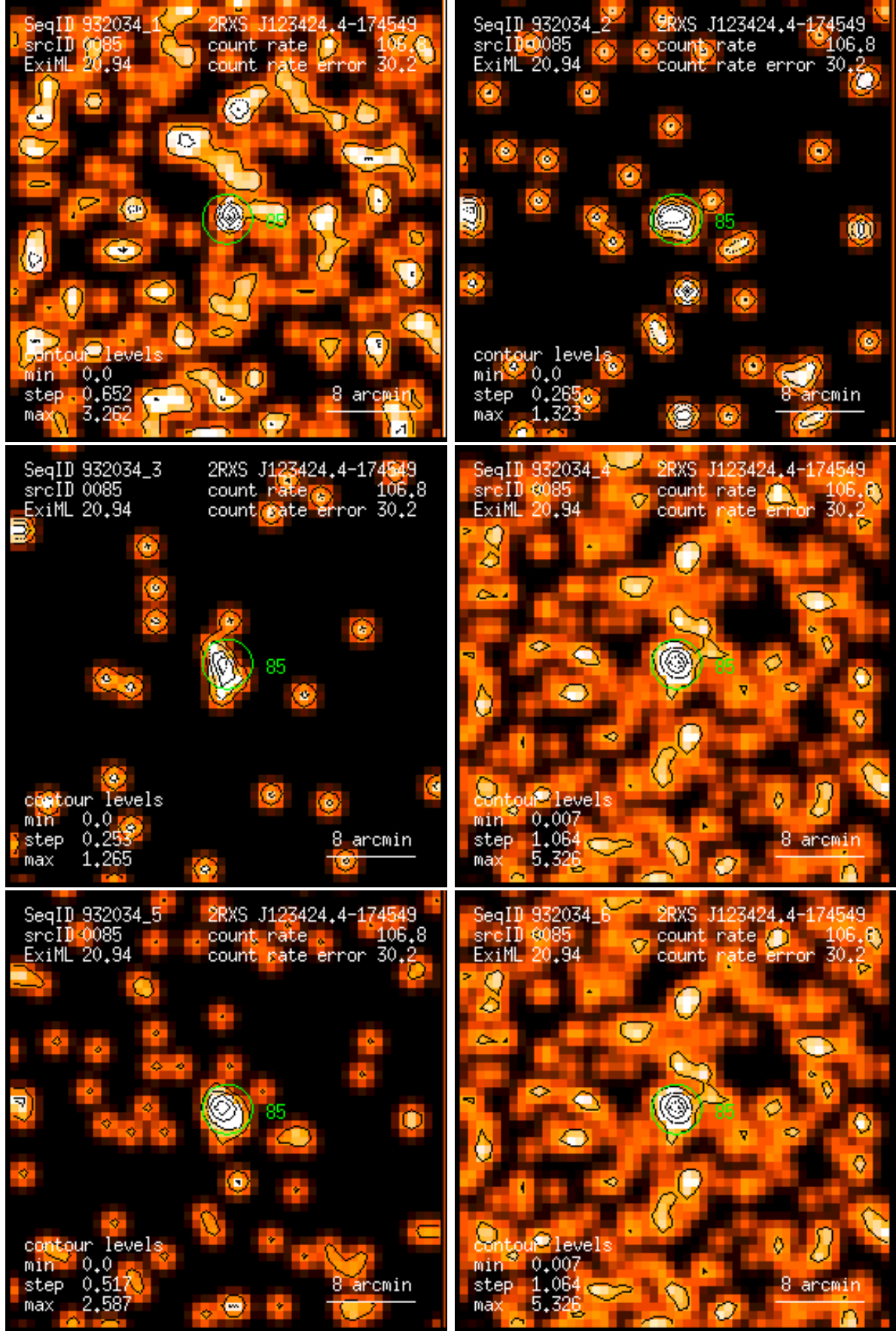
Figure 85: RASS 932034: detection 0085: band rate images, Gaussian filter: (1) PSPC channels 11 – 41, (2) 52 – 90, (3) 91 – 201, (4) 11 – 235, (5) 52 – 201, (6) 11 – 201. Broad band rates in counts/ks. Band rate contour levels in counts/ks/arcmin 2 .
