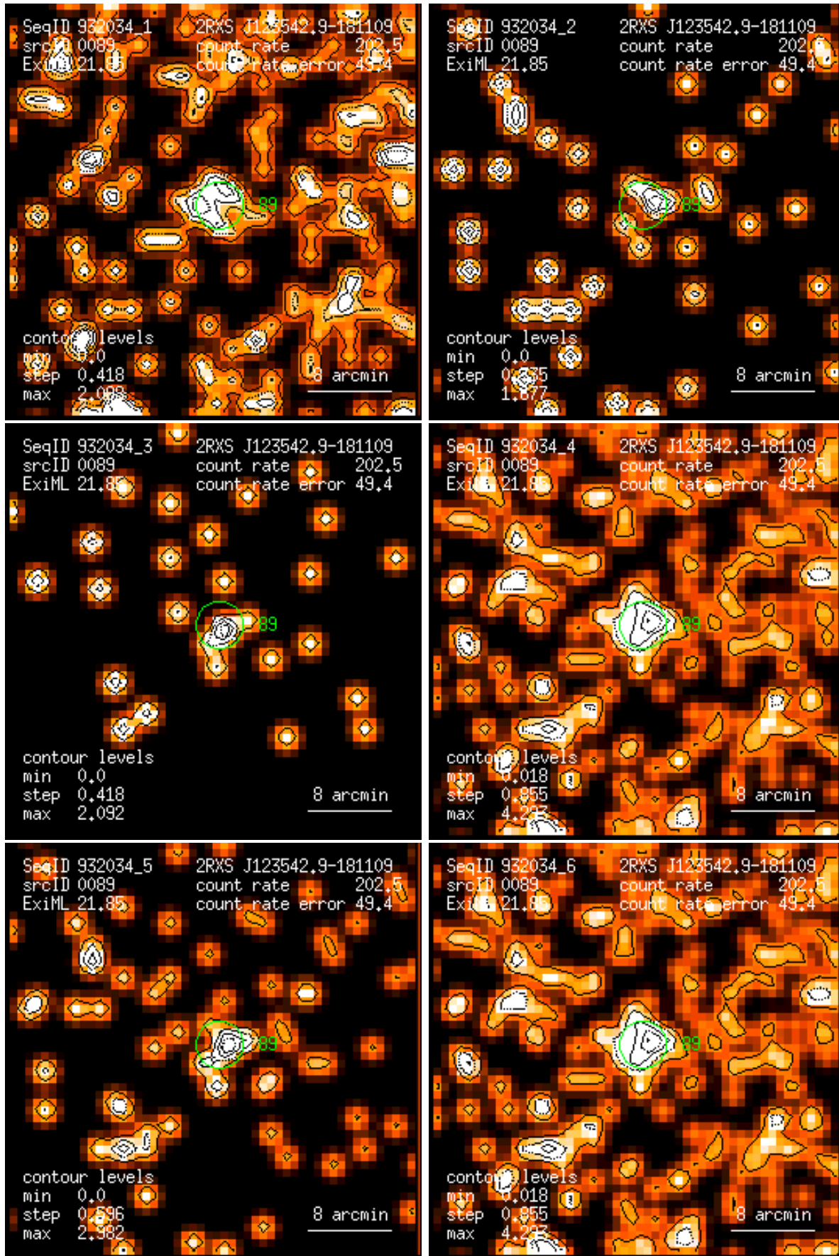
Figure 89: RASS 932034: detection 0089: band rate images, Gaussian filter: (1) PSPC channels 11 – 41, (2) 52 – 90, (3) 91 – 201, (4) 11 – 235, (5) 52 – 201, (6) 11 – 201. Broad band rates in counts/ks. Band rate contour levels in counts/ks/arcmin 2 .
