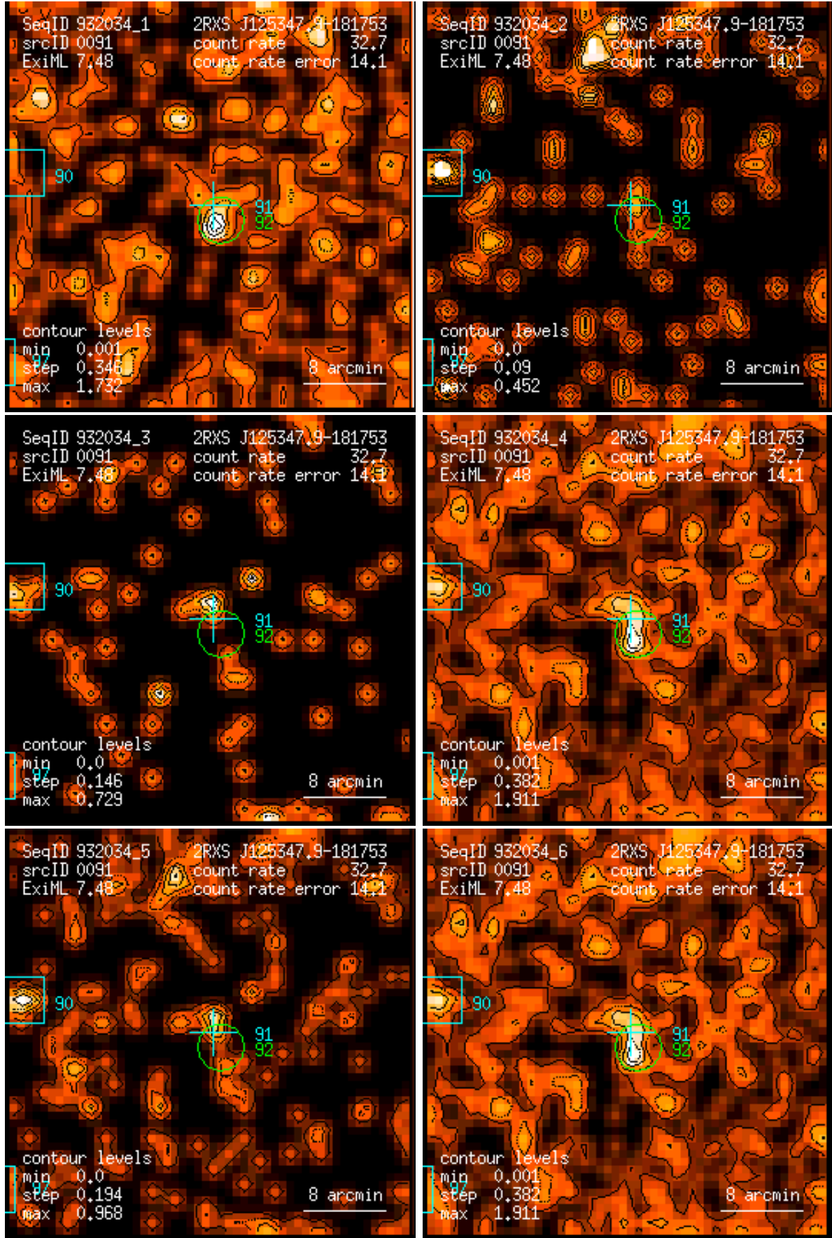
Figure 91: RASS 932034: detection 0091: band rate images, Gaussian filter: (1) PSPC channels 11 – 41, (2) 52 – 90, (3) 91 – 201, (4) 11 – 235, (5) 52 – 201, (6) 11 – 201. Broad band rates in counts/ks. Band rate contour levels in counts/ks/arcmin 2 .
