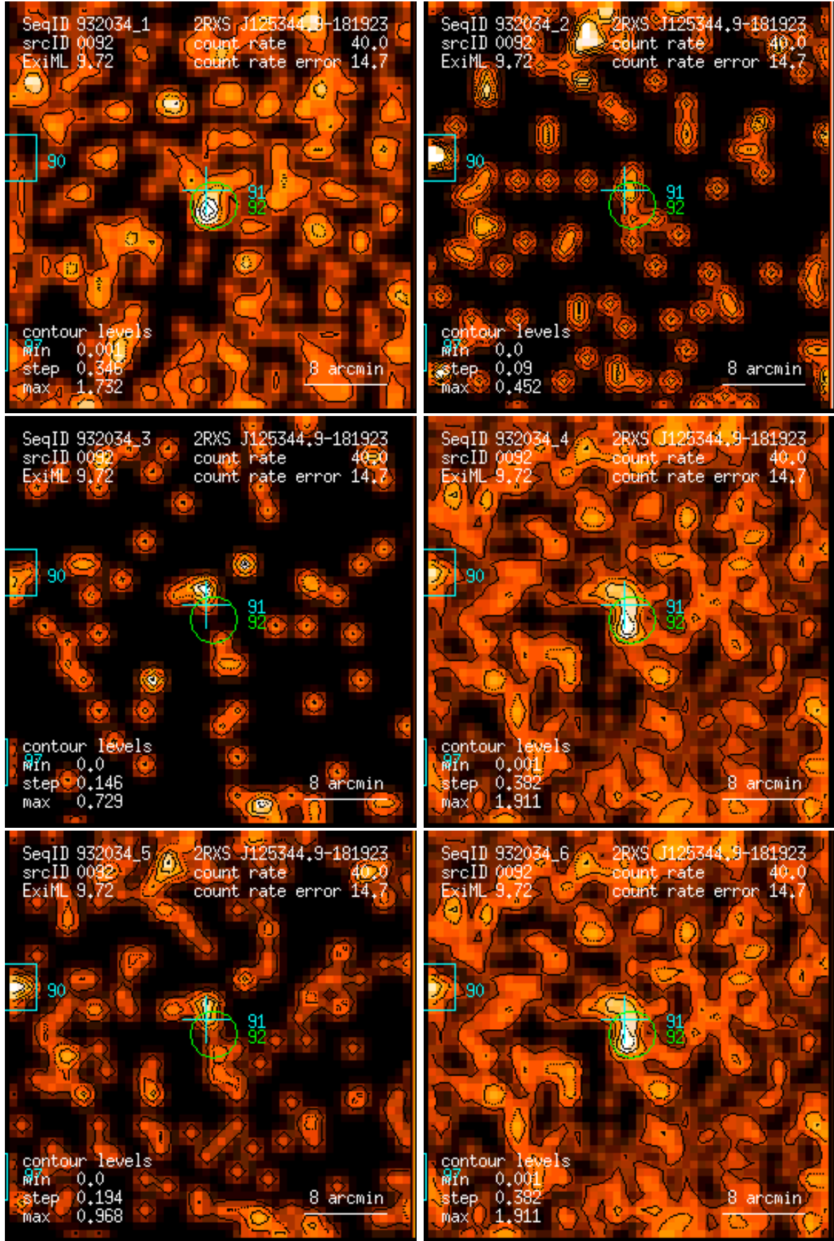
Figure 92: RASS 932034: detection 0092: band rate images, Gaussian filter: (1) PSPC channels 11 – 41, (2) 52 – 90, (3) 91 – 201, (4) 11 – 235, (5) 52 – 201, (6) 11 – 201. Broad band rates in counts/ks. Band rate contour levels in counts/ks/arcmin 2 .
