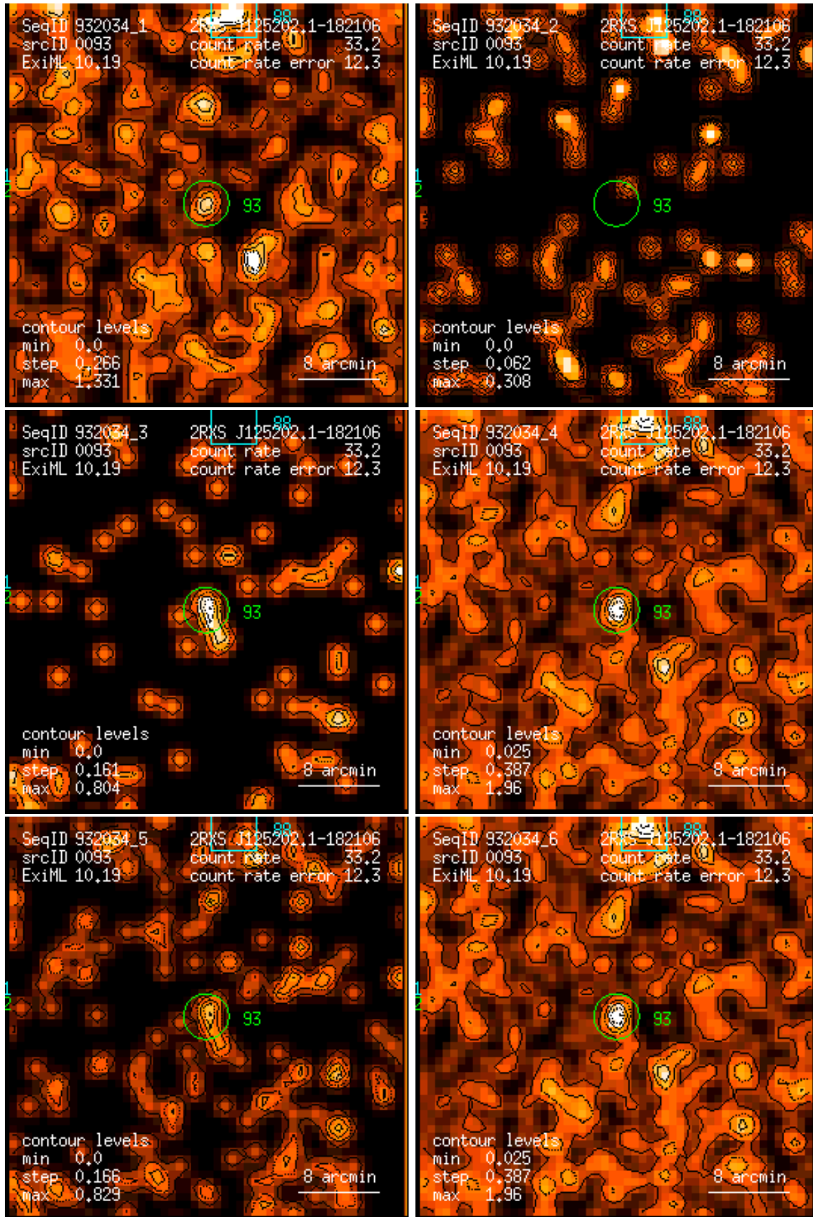
Figure 93: RASS 932034: detection 0093: band rate images, Gaussian filter: (1) PSPC channels 11 – 41, (2) 52 – 90, (3) 91 – 201, (4) 11 – 235, (5) 52 – 201, (6) 11 – 201. Broad band rates in counts/ks. Band rate contour levels in counts/ks/arcmin 2 .
