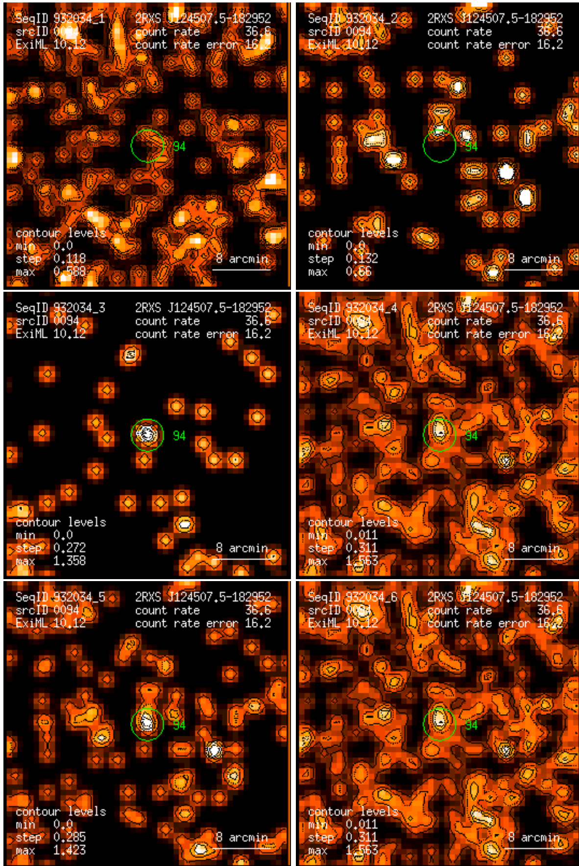
Figure 94: RASS 932034: detection 0094: band rate images, Gaussian filter: (1) PSPC channels 11 – 41, (2) 52 – 90, (3) 91 – 201, (4) 11 – 235, (5) 52 – 201, (6) 11 – 201. Broad band rates in counts/ks. Band rate contour levels in counts/ks/arcmin 2 .
