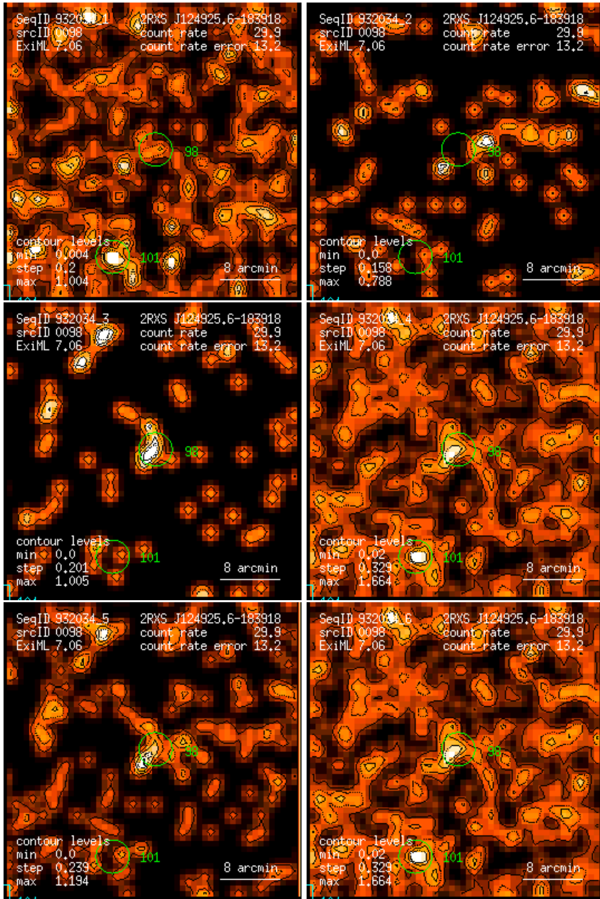
Figure 98: RASS 932034: detection 0098: band rate images, Gaussian filter: (1) PSPC channels 11 – 41, (2) 52 – 90, (3) 91 – 201, (4) 11 – 235, (5) 52 – 201, (6) 11 – 201. Broad band rates in counts/ks. Band rate contour levels in counts/ks/arcmin 2 .
