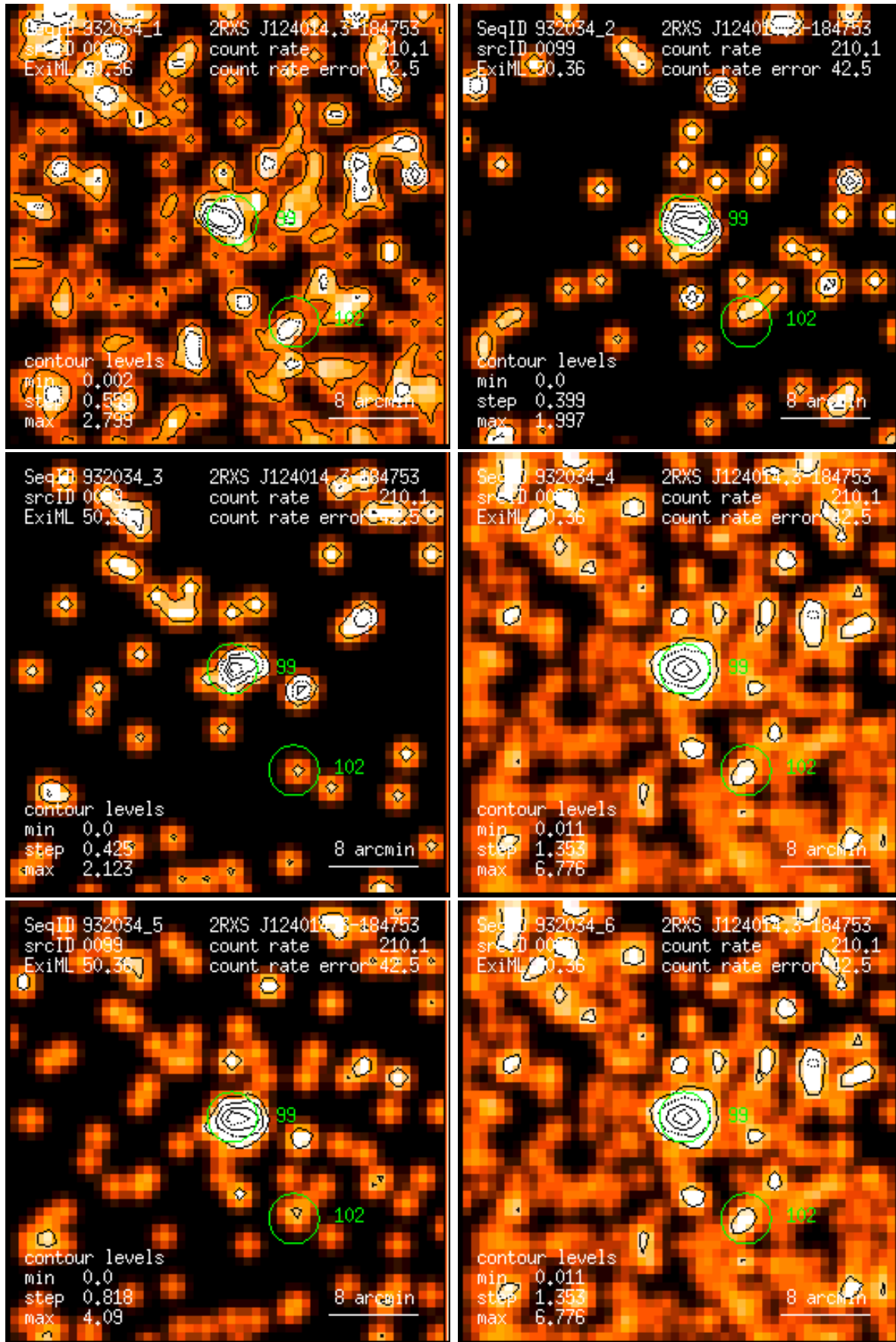
Figure 99: RASS 932034: detection 0099: band rate images, Gaussian filter: (1) PSPC channels 11 – 41, (2) 52 – 90, (3) 91 – 201, (4) 11 – 235, (5) 52 – 201, (6) 11 – 201. Broad band rates in counts/ks. Band rate contour levels in counts/ks/arcmin 2 .
