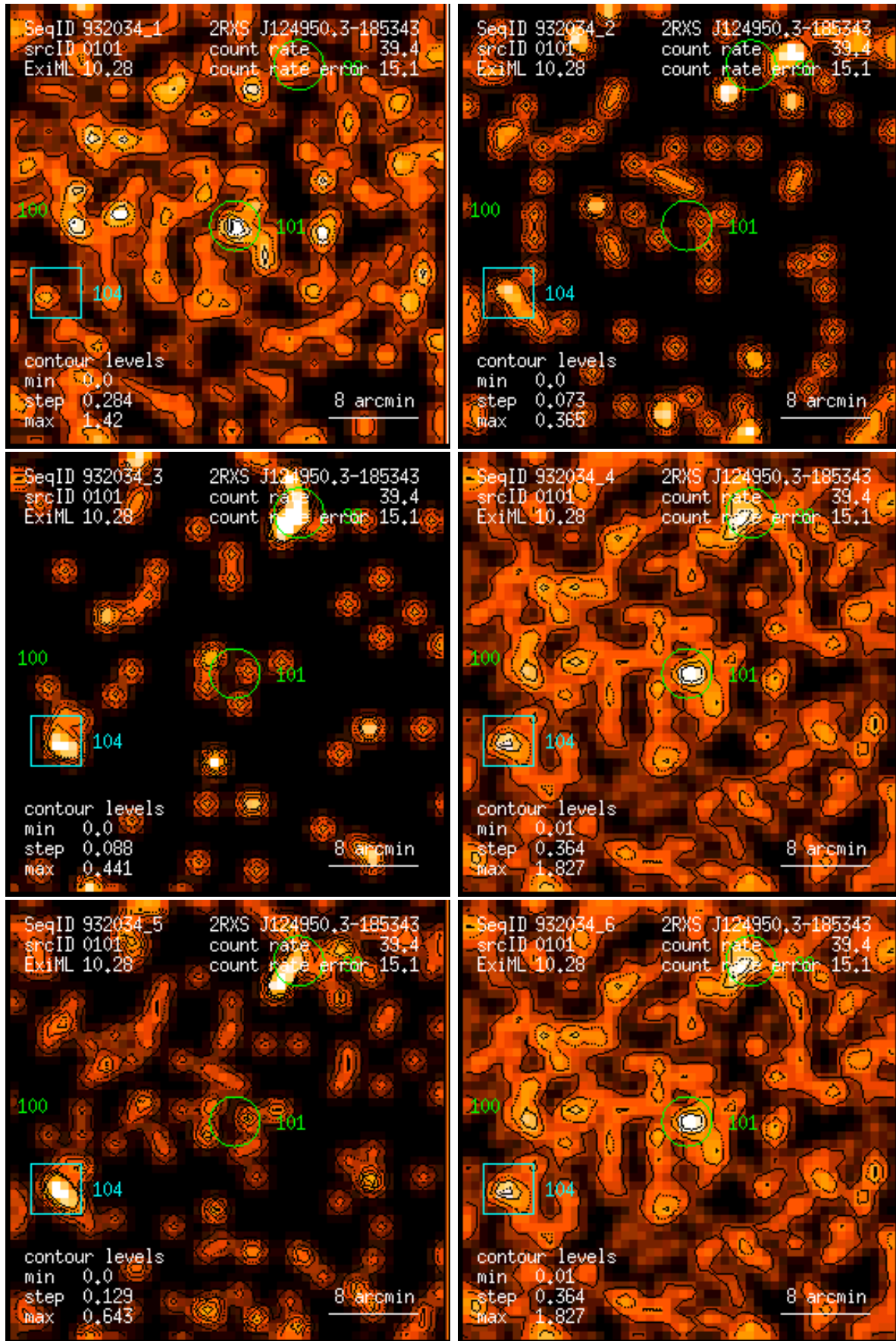
Figure 101: RASS 932034: detection 0101: band rate images, Gaussian filter: (1) PSPC channels 11 – 41, (2) 52 – 90, (3) 91 – 201, (4) 11 – 235, (5) 52 – 201, (6) 11 – 201. Broad band rates in counts/ks. Band rate contour levels in counts/ks/arcmin 2 .
