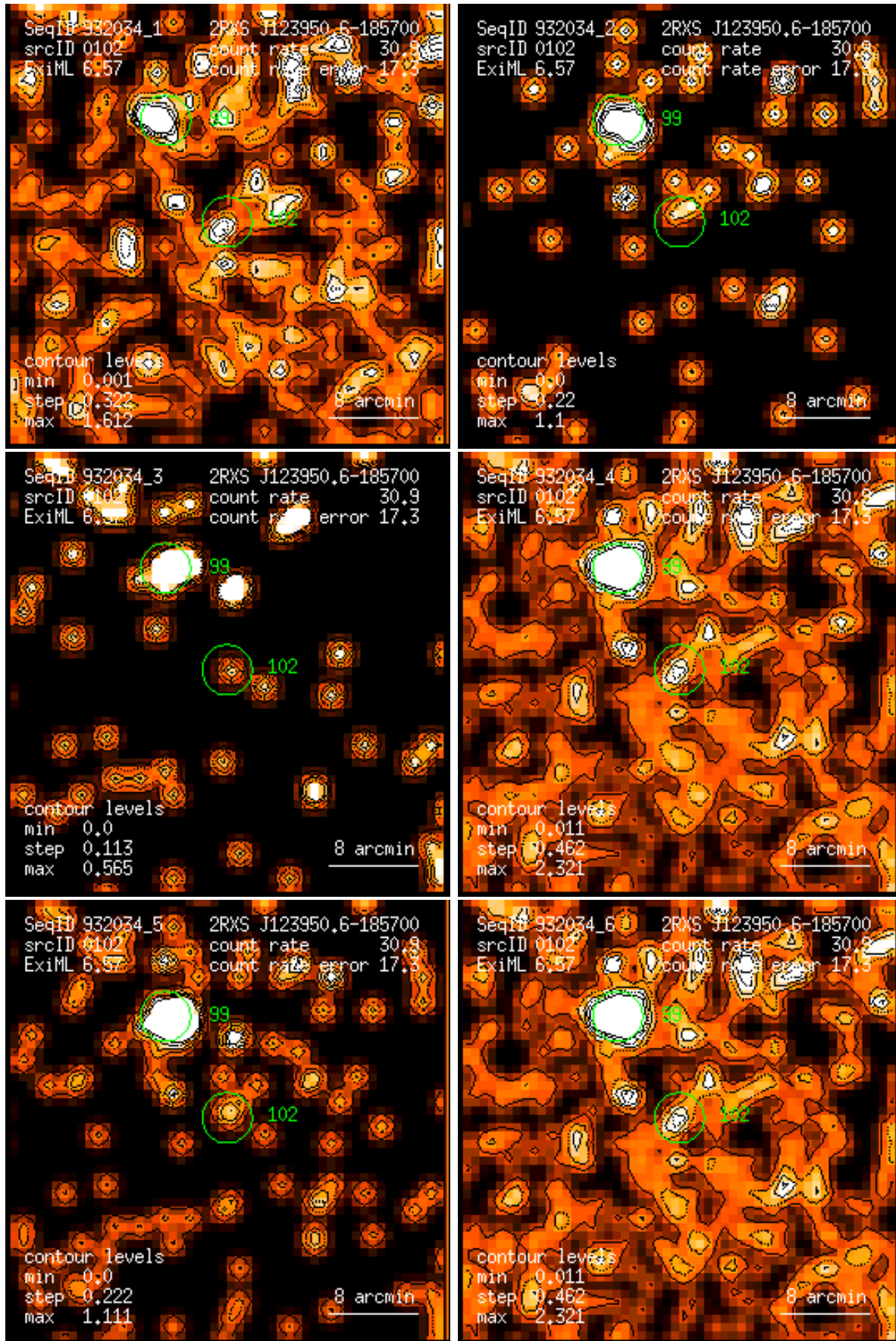
Figure 102: RASS 932034: detection 0102: band rate images, Gaussian filter: (1) PSPC channels 11 – 41, (2) 52 – 90, (3) 91 – 201, (4) 11 – 235, (5) 52 – 201, (6) 11 – 201. Broad band rates in counts/ks. Band rate contour levels in counts/ks/arcmin 2 .
