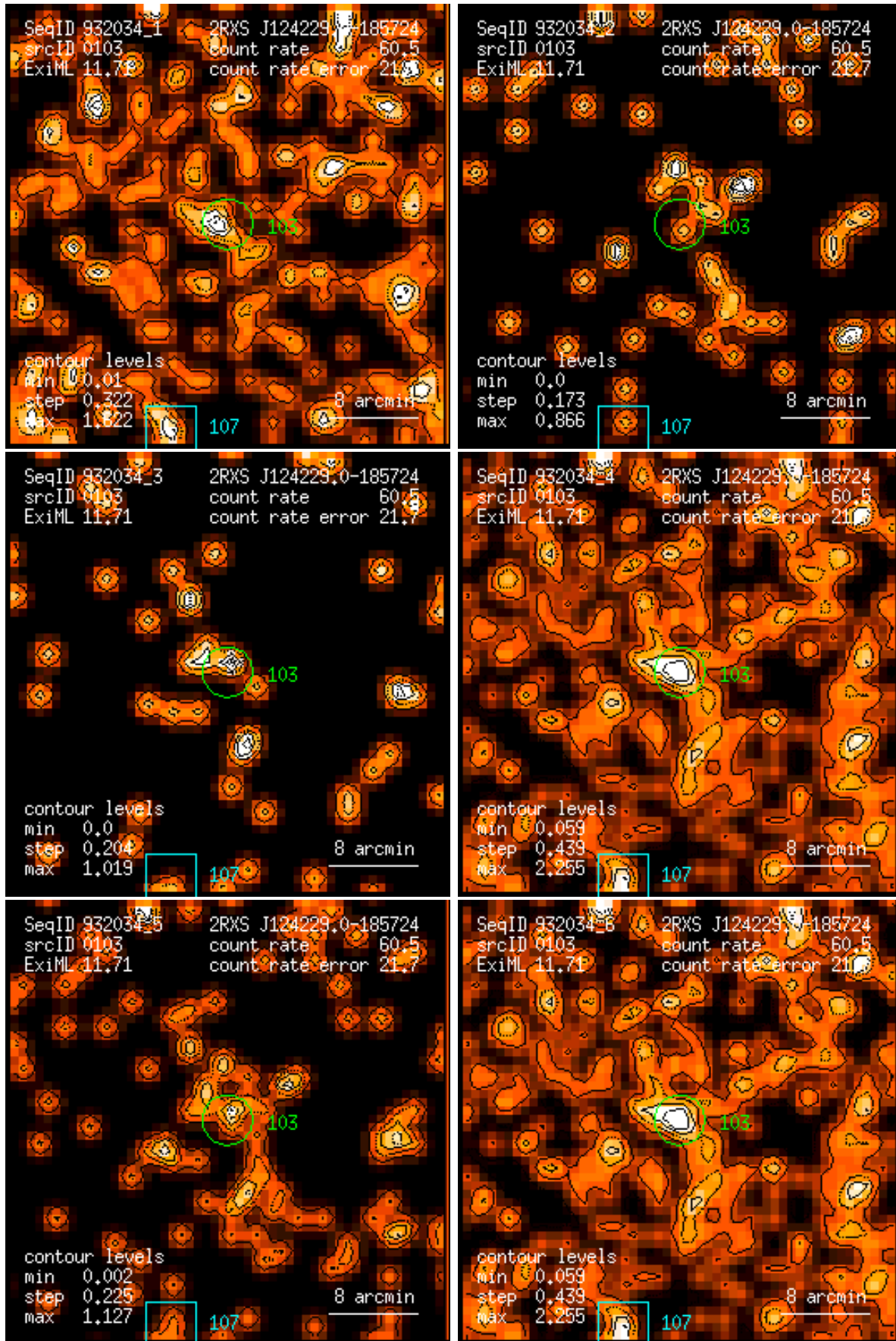
Figure 103: RASS 932034: detection 0103: band rate images, Gaussian filter: (1) PSPC channels 11 – 41, (2) 52 – 90, (3) 91 – 201, (4) 11 – 235, (5) 52 – 201, (6) 11 – 201. Broad band rates in counts/ks. Band rate contour levels in counts/ks/arcmin 2 .
