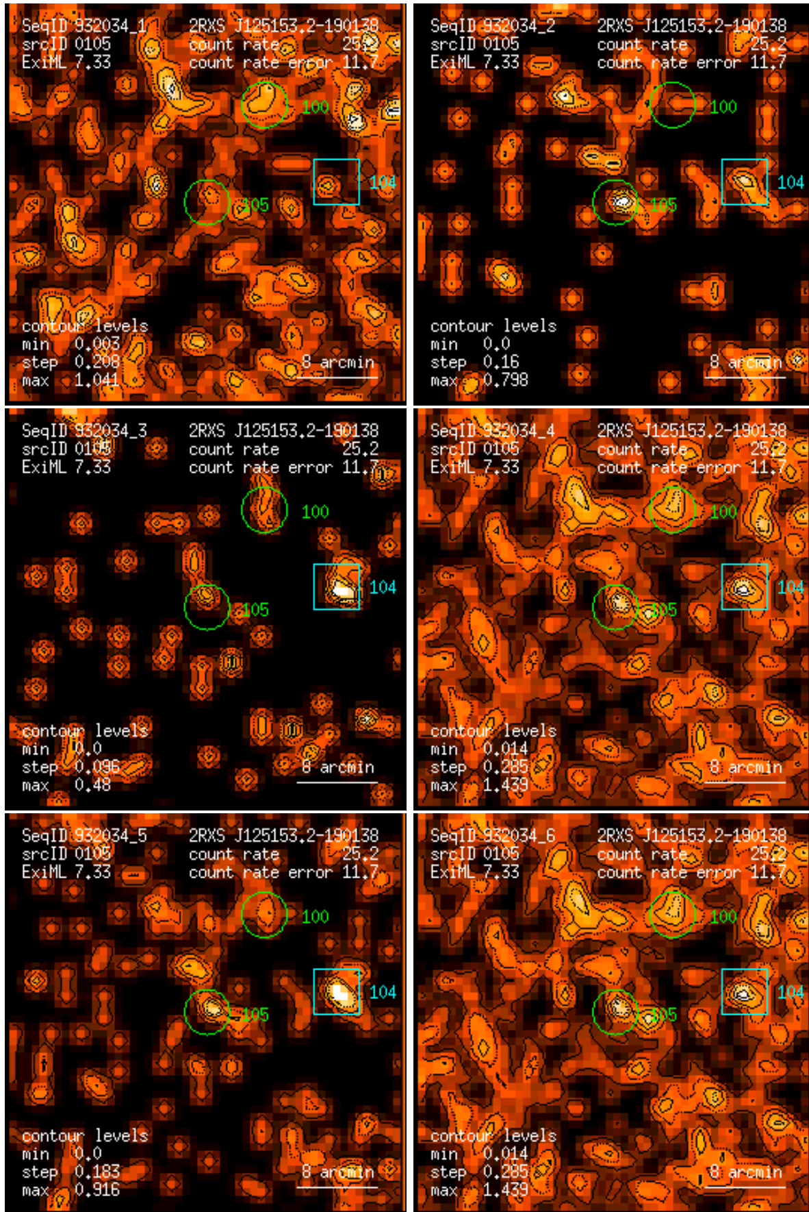
Figure 105: RASS 932034: detection 0105: band rate images, Gaussian filter: (1) PSPC channels 11 – 41, (2) 52 – 90, (3) 91 – 201, (4) 11 – 235, (5) 52 – 201, (6) 11 – 201. Broad band rates in counts/ks. Band rate contour levels in counts/ks/arcmin 2 .
