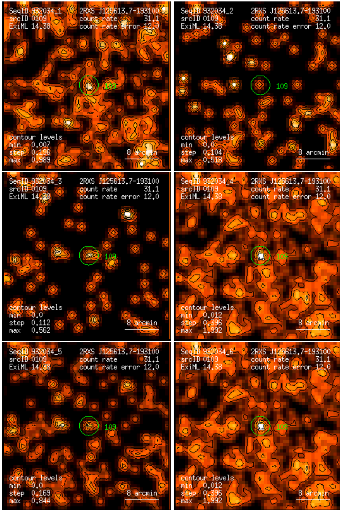
Figure 109: RASS 932034: detection 0109: band rate images, Gaussian filter: (1) PSPC channels 11 – 41, (2) 52 – 90, (3) 91 – 201, (4) 11 – 235, (5) 52 – 201, (6) 11 – 201. Broad band rates in counts/ks. Band rate contour levels in counts/ks/arcmin 2 .
