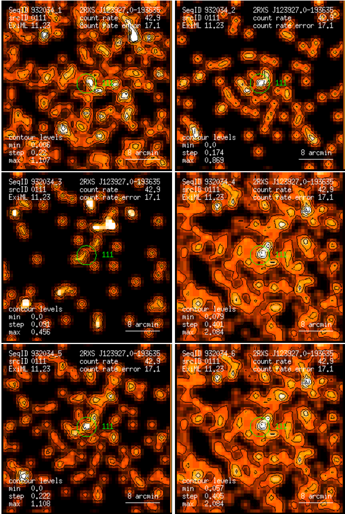
Figure 111: RASS 932034: detection 0111: band rate images, Gaussian filter: (1) PSPC channels 11 – 41, (2) 52 – 90, (3) 91 – 201, (4) 11 – 235, (5) 52 – 201, (6) 11 – 201. Broad band rates in counts/ks. Band rate contour levels in counts/ks/arcmin 2 .
