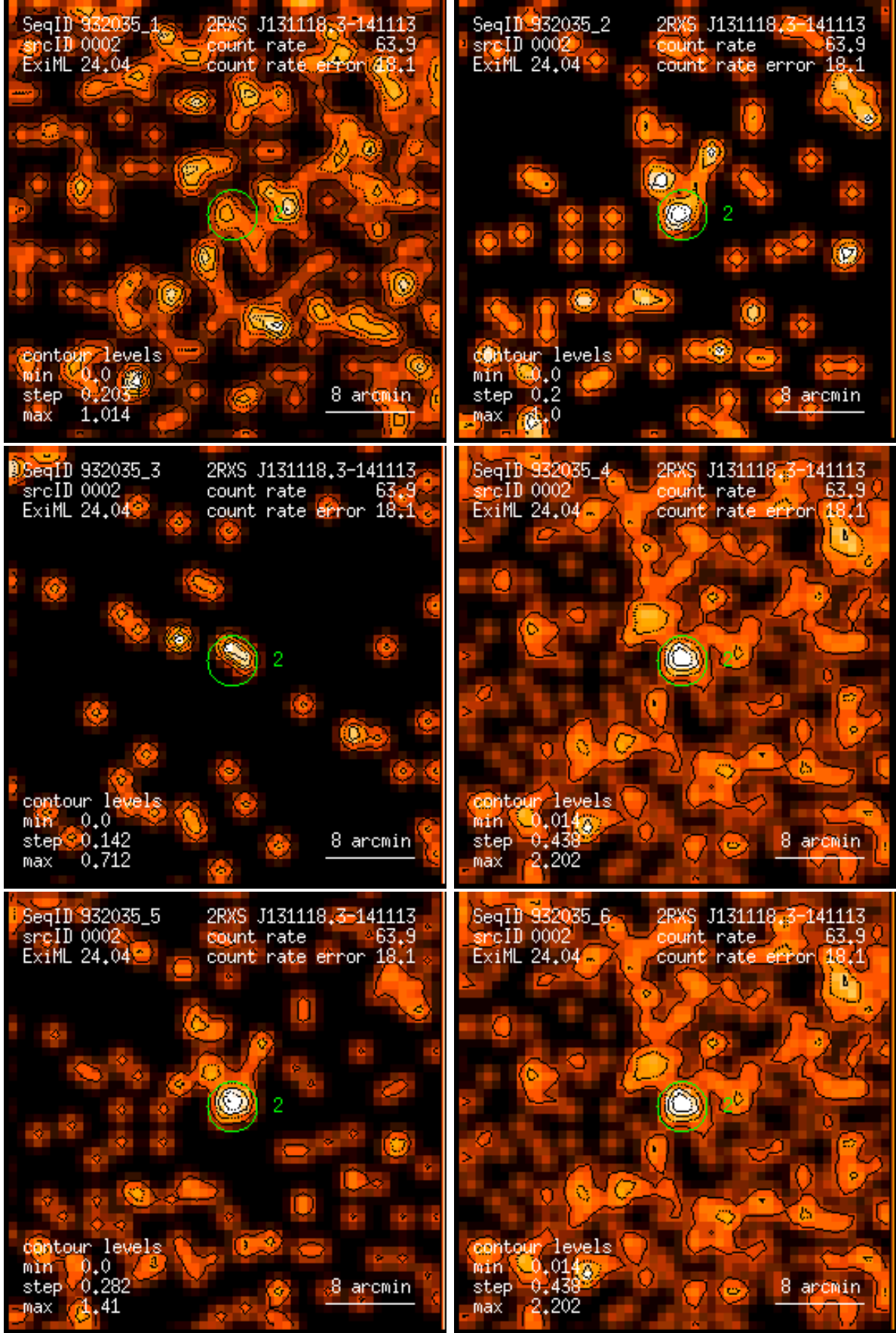
Figure 2: RASS 932035: detection 0002: band rate images, Gaussian filter: (1) PSPC channels 11 – 41, (2) 52 – 90, (3) 91 – 201, (4) 11 – 235, (5) 52 – 201, (6) 11 – 201. Broad band rates in counts/ks. Band rate contour levels in counts/ks/arcmin 2 .
