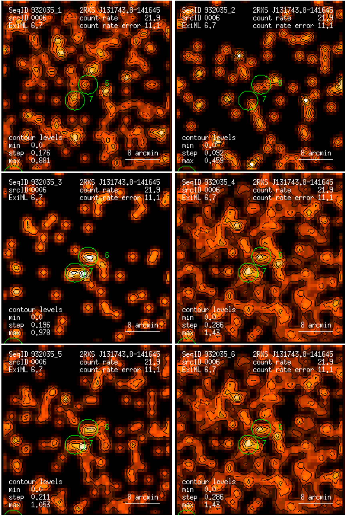
Figure 6: RASS 932035: detection 0006: band rate images, Gaussian filter: (1) PSPC channels 11 – 41, (2) 52 – 90, (3) 91 – 201, (4) 11 – 235, (5) 52 – 201, (6) 11 – 201. Broad band rates in counts/ks. Band rate contour levels in counts/ks/arcmin 2 .
