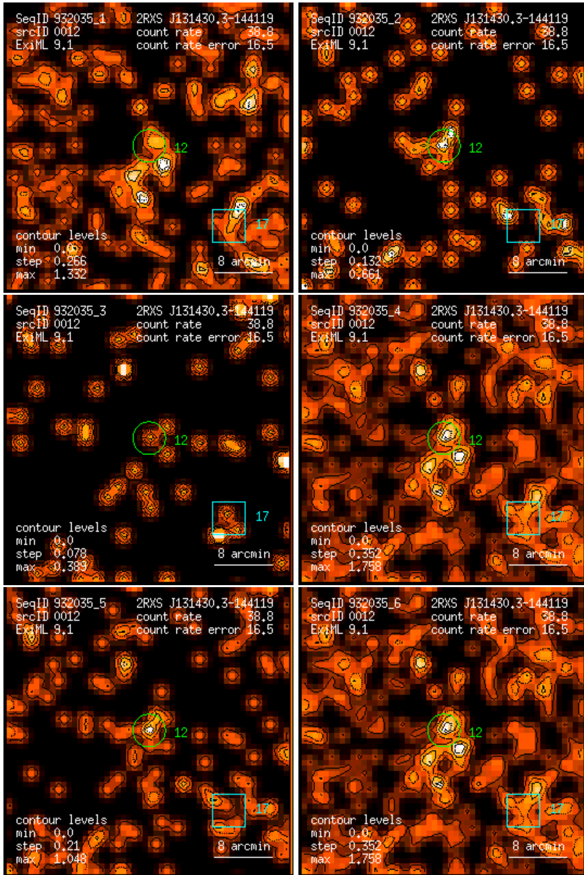
Figure 12: RASS 932035: detection 0012: band rate images, Gaussian filter: (1) PSPC channels 11 – 41, (2) 52 – 90, (3) 91 – 201, (4) 11 – 235, (5) 52 – 201, (6) 11 – 201. Broad band rates in counts/ks. Band rate contour levels in counts/ks/arcmin 2 .
