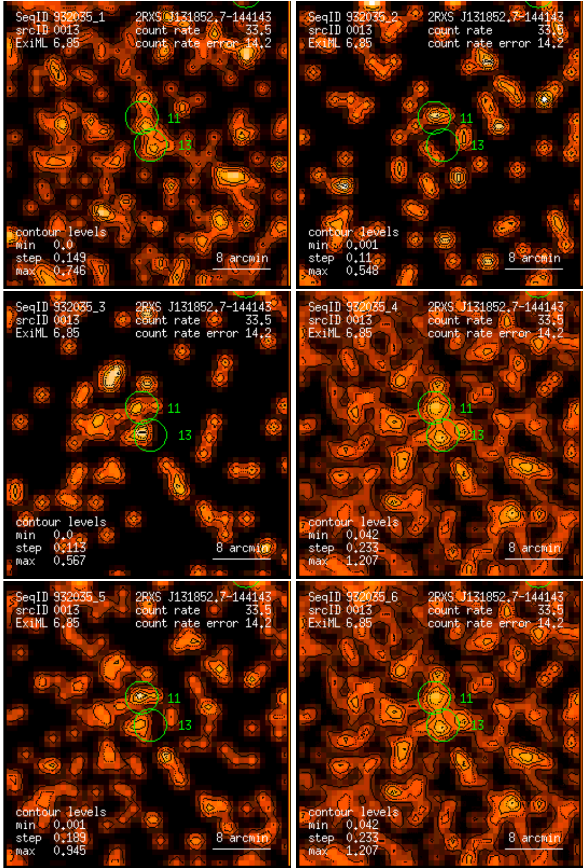
Figure 13: RASS 932035: detection 0013: band rate images, Gaussian filter: (1) PSPC channels 11 – 41, (2) 52 – 90, (3) 91 – 201, (4) 11 – 235, (5) 52 – 201, (6) 11 – 201. Broad band rates in counts/ks. Band rate contour levels in counts/ks/arcmin 2 .
