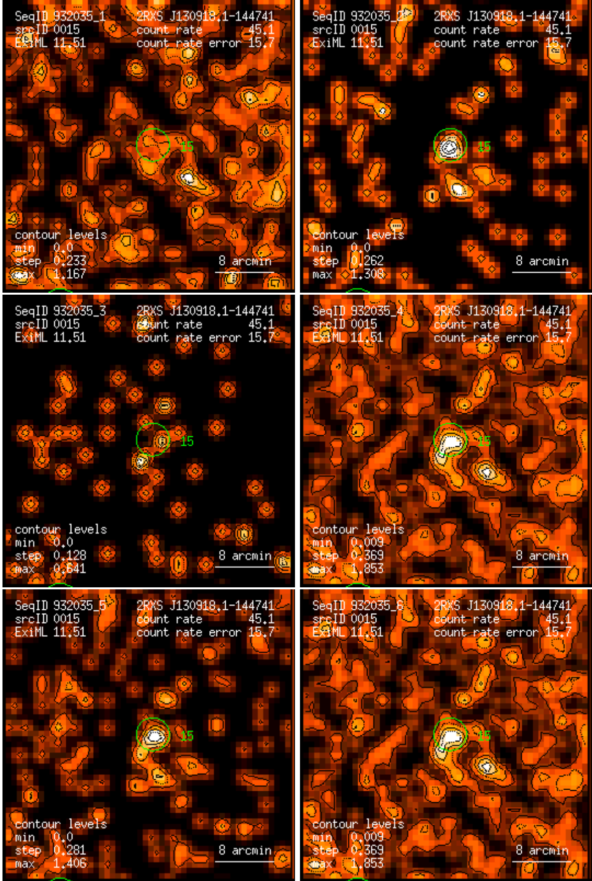
Figure 15: RASS 932035: detection 0015: band rate images, Gaussian filter: (1) PSPC channels 11 – 41, (2) 52 – 90, (3) 91 – 201, (4) 11 – 235, (5) 52 – 201, (6) 11 – 201. Broad band rates in counts/ks. Band rate contour levels in counts/ks/arcmin 2 .
